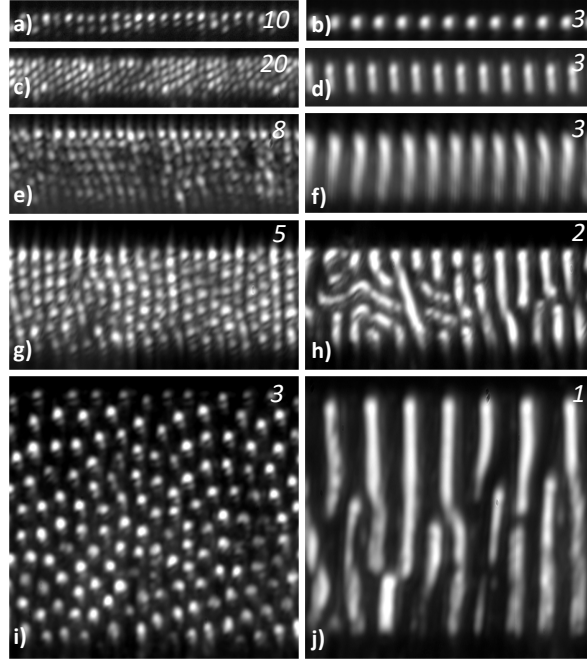
Figure 3: Rod-like (left column) and lamellar (right column) patterns in eutectic SCN-DC samples of various thicknesses. From top to bottom, \delta = 30, 60, 100, 140 , and 350 \mu\text{m} . Pulling velocities are indicated in terms of V/V_0 , with V_0 = 0.0035 \mu\text{ms}^{-1} (top right corner of each panel). d) Same sample as in Fig. 1b. Horizontal dimension: 370 \mu\text{m} [a) to f)]; 410 \mu\text{m} [g) to j)].
