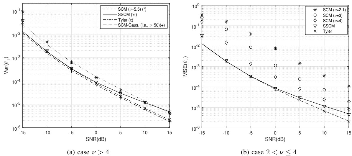
Fig. 2. Theoretical asymptotic variance \frac{r_{\hat{\theta}}}{T} and MSEs (with 2000 Monte Carlo runs) of conventional MUSIC algorithm based on SCM, SSCM and Tyler's M estimate versus SNR for circular complex Student's t -distributed data (with T = 500 ) for either \nu > 4 or 2 < \nu \leq 4 and N = 6 .
