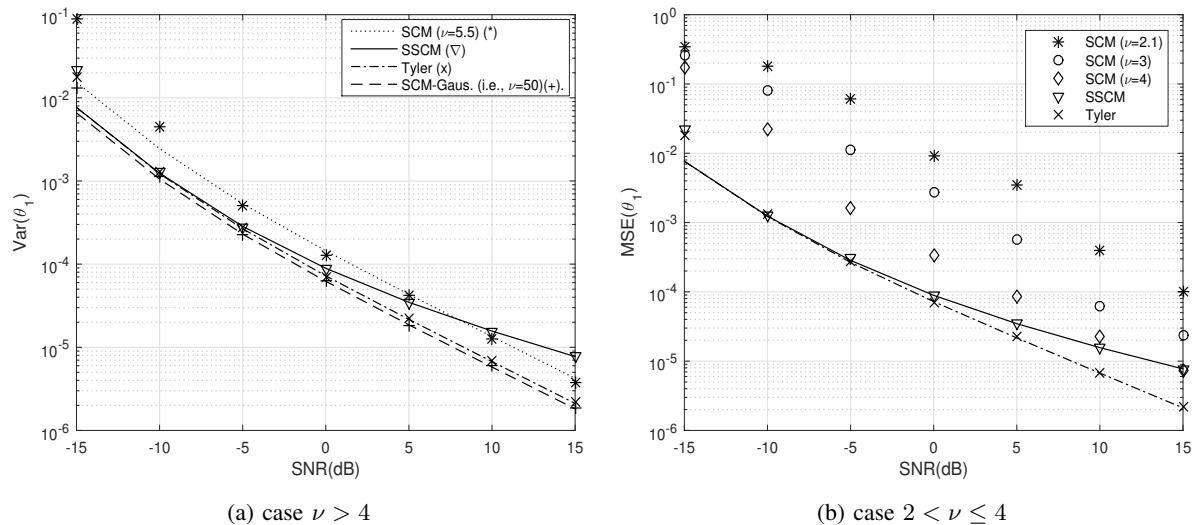
Fig. 3. Theoretical asymptotic variance \frac{r_{\hat{\theta}}}{T} and MSEs (with 2000 Monte Carlo runs) of NC MUSIC algorithm based on SCM, SSCM and Tyler's M estimate versus SNR for NC complex Student's t -distributed data (with T = 500 ) for either \nu > 4 or 2 < \nu \leq 4 with \phi = \pi/3 and N = 6
