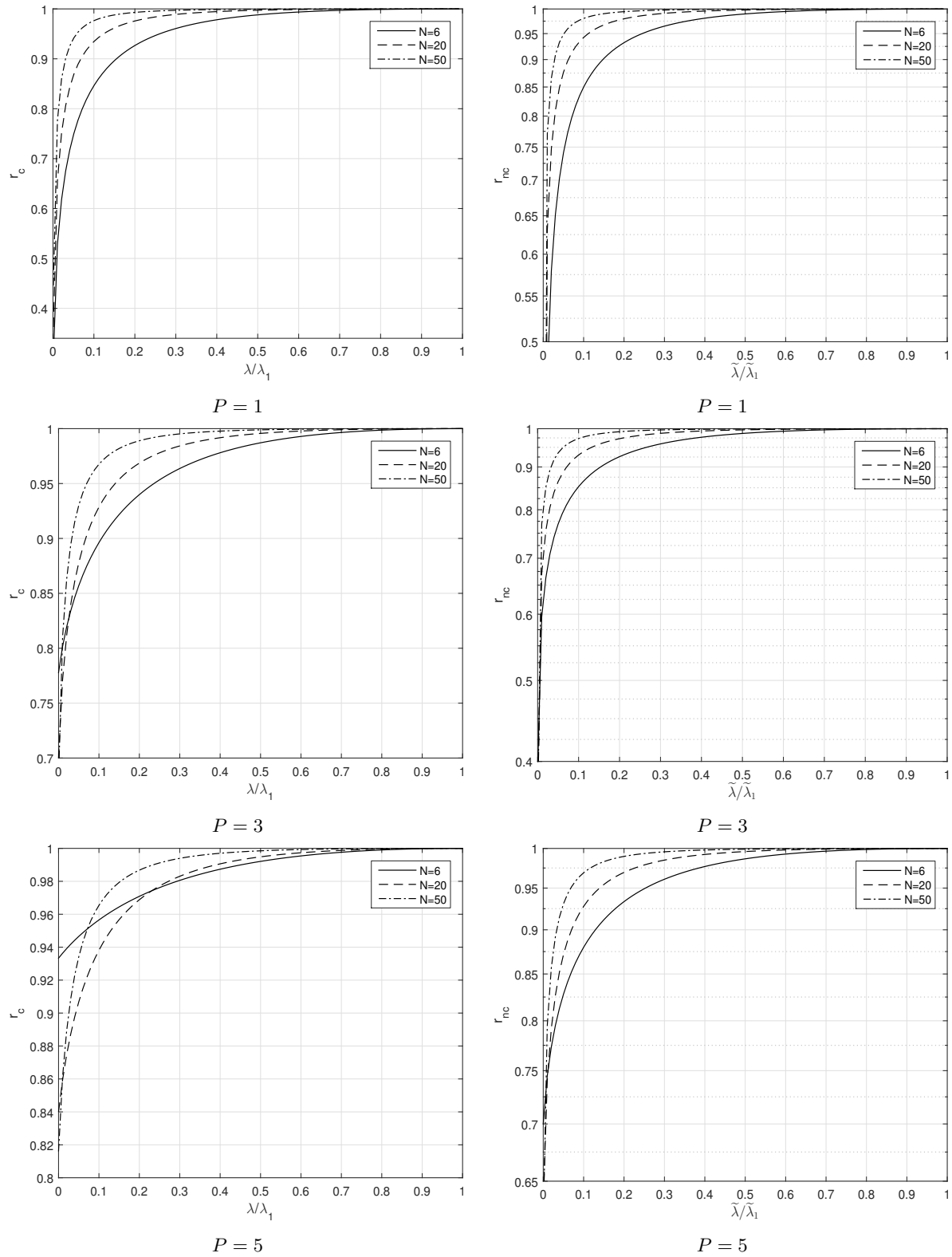
Fig. 1. Ratios r_c and r_{nc} versus respectively \lambda/\lambda_1 and \tilde{\lambda}/\tilde{\lambda}_1 for different values of N and P = 1, 3, 5 .
