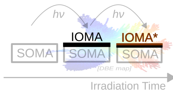
Fig. 3. Possible evolution process leading to the formation of IOMA from SOMA. The upper 0.1 \mu\text{m} layer of the SOMA are UV irradiated, leading to the formation of the first IOMA molecules (dark). Once formed, these IOMA first-generation molecules are UV irradiated, leading to an evolved generation of IOMA (brown). This evolution is visible in the gradient of #C, #N, and DBE of elementary maps (Figure B.5).
