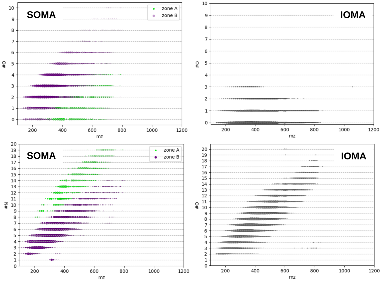
Fig. B.1. Evolution of O or N elements as a function of m/z for SOMA or IOMA for (A) all attributions or for CHNO or CHN groups only.
