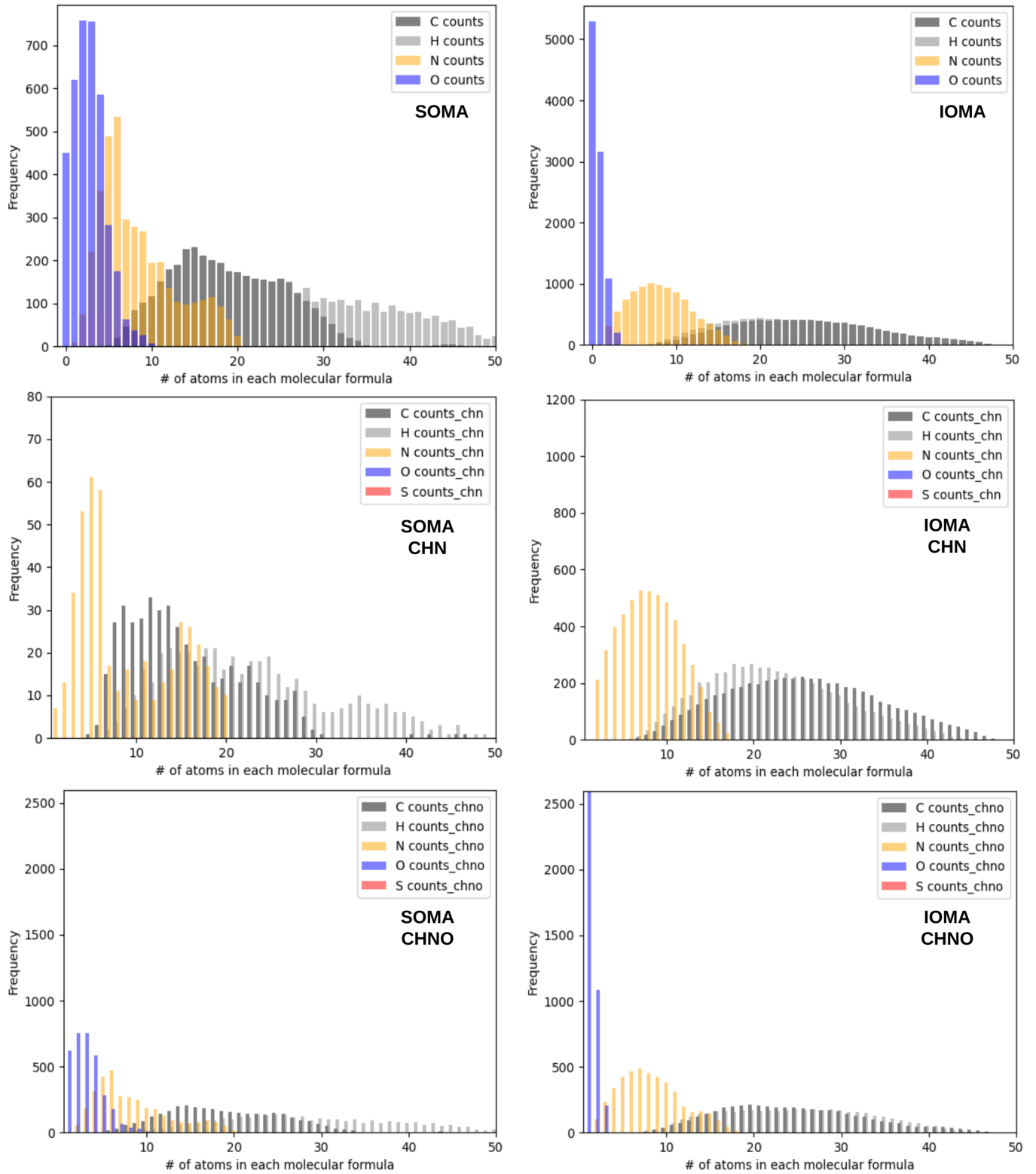
Fig. B.2. Frequencies of atoms in each molecular formula for all attributions, CHNO, or CHN (groups for SOMA and IOMA).
