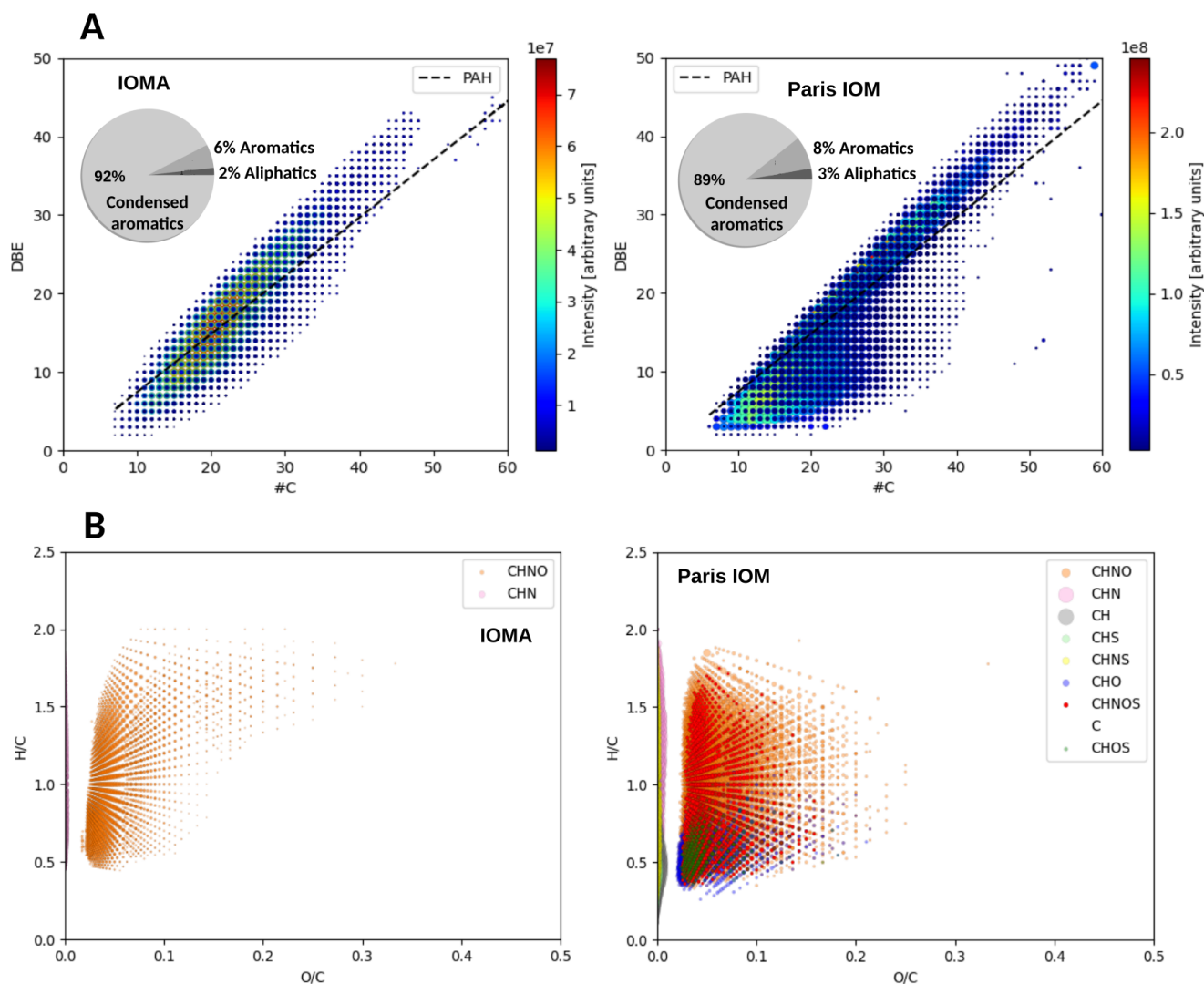
Fig. 4. IOMA versus IOM of Paris. (A) Representations of DBE versus the number of carbon ( \#C ) for IOMA and IOM, with X_C pie charts showing attribution repartitions between aliphatic, aromatic, and condensed aromatic structures. (B) Van Krevelen H/C versus O/C for attributions identified in IOMA and IOM of Paris meteorite. For the Paris meteorite, data were reproduced from Danger et al. (Danger et al. 2020).
