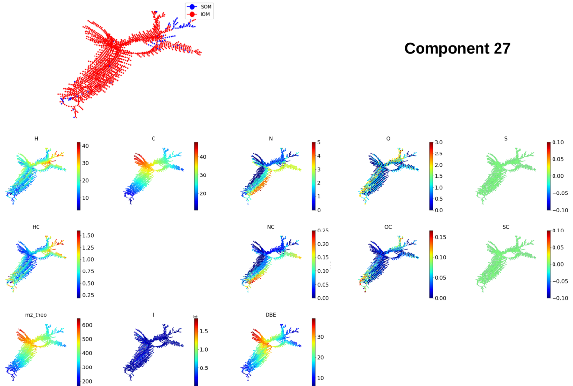
Fig. B.7. Element maps of SOM-IOM transition graph components number 38 (A) and number 27 (B) for Paris meteorite network. Article number, page 18 of 18
