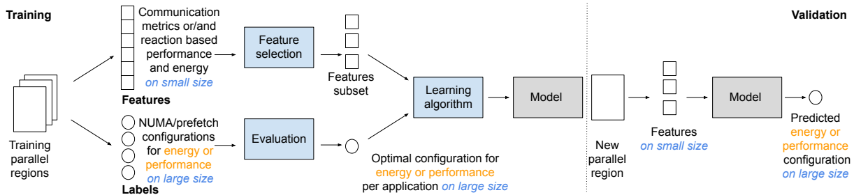
Fig. 6. ML workflow when predicting optimizations from small size to large size. Left: model training. Right: model validation. The model predicts NUMA/prefetch configurations for large size by only measuring a few features on small size. The same workflow is used for performance or energy models.
