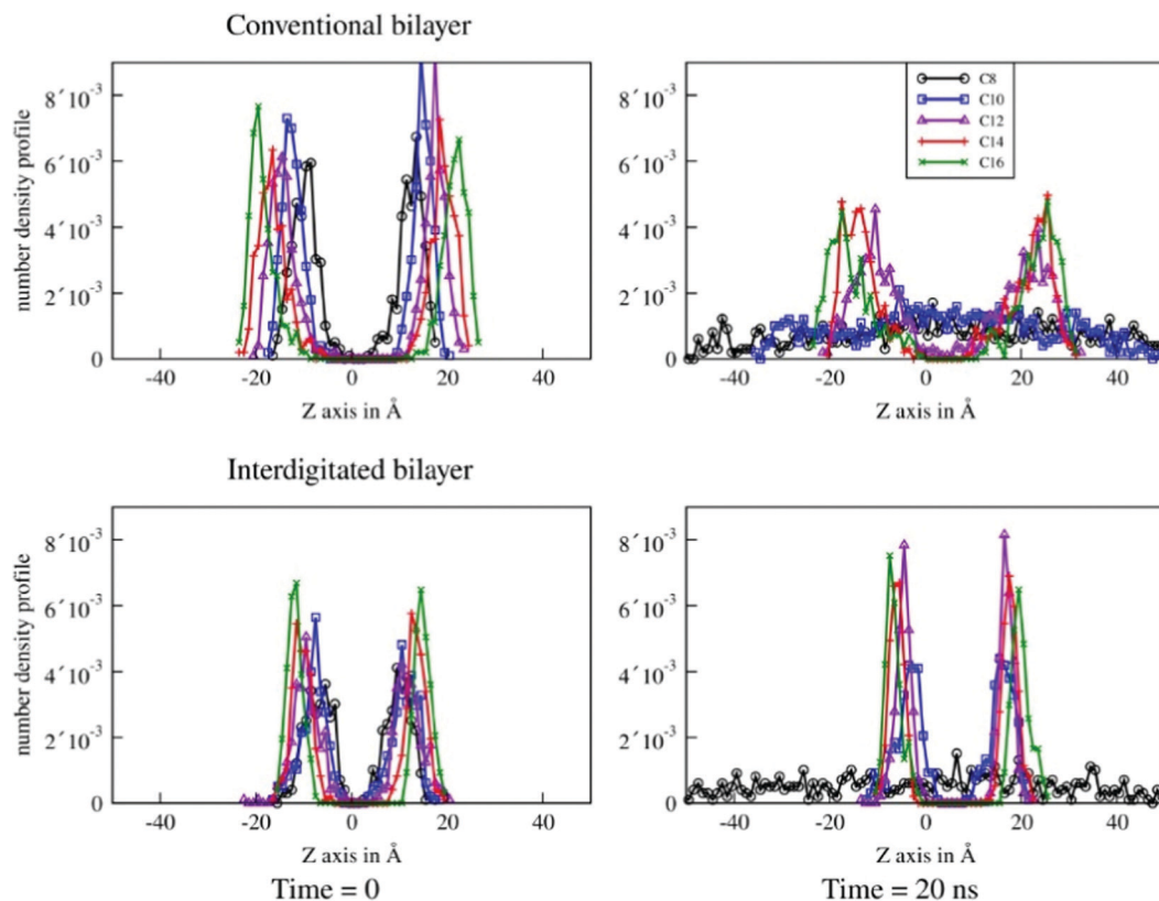
Fig. 9 Sulfur atom, number density profile ( \text{Atom \AA}^{-3} ) along the Z axis.
