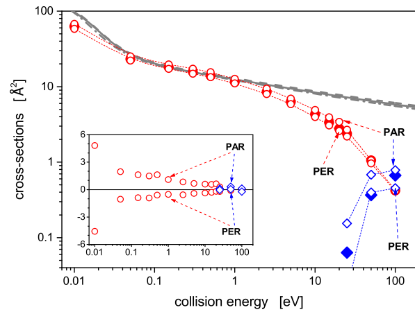
Figure 7. Comparison of type 1 momentum-transfer cross-sections (circles) and collision-induced dissociation cross-sections (diamonds) as obtained for N_2^+(j=0,v=0)/He collisions assuming angular momentum of N_2^+ perpendicularly (PER) and/or parallelly (PAR) aligned to the collision axis (open symbols), and non-aligned (full symbols). For comparison, inverse-method cross-sections are also depicted as grey lines in the background. In the inset, deviations of the PER/PAR cross-sections from the cross-sections calculated for non-aligned N_2^+ are depicted.
