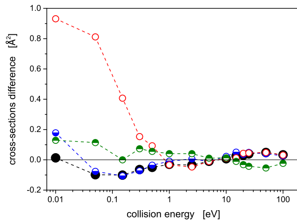
Figure 4. Deviations between type 2 and type 1 momentum-transfer cross-sections ( MTCS2-MTCS1 ) of the NRS channel (Eq. (1)) as calculated at the MCSCF/avqz(spdf) level for selected rotational-vibrational states of the N_2^+ ion. The symbols used are the same as in Fig. 2, the connecting lines are added to guide eyes.
