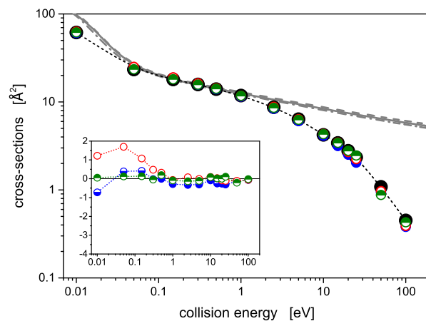
Figure 2. Type 1 momentum-transfer cross-sections (MTCS1) of N_2^+(j, v) + He \rightarrow N_2^+ + He collisions as calculated for selected rotational-vibrational states of the N_2^+ ion at the MCSCF/avqz(spdf) level: full circles j=0, v=0 , upper half-filled circles j=0, v=1 , lower half-filled circles j=0, v=10 , and open circles j=36, v=0 . Inverse-method values derived from selected experimental data are also included as gray lines in the background (with the line patterns used as in Fig. 1). In the inset, deviations of the MTCS1 calculated for the vibrationally and/or rotationally excited N_2^+ ions from the MTCS1 values obtained for j=0, v=0 are depicted.
