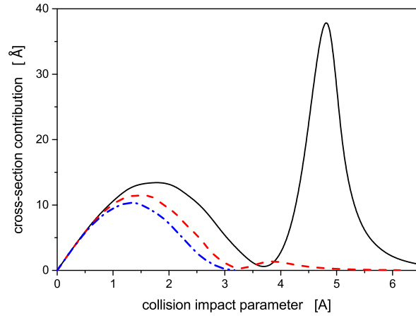
Figure 3. Contributions of particular impact-parameters to type 1 momentum-transfer cross-sections, 2\pi b\Delta\sigma_{\text{NRS}}^{(\text{MT1})}(b) (see Eq. (7)), of N_2^+(j=0, v=0)+\text{He} \rightarrow N_2^++\text{He} collisions as calculated at the MCSCF/avqz(spdf) level for selected collision energies: full line E_{\text{coll}} = 0.01 eV, dashed line E_{\text{coll}} = 0.05 eV, and dash-dotted line E_{\text{coll}} = 0.15 eV.
