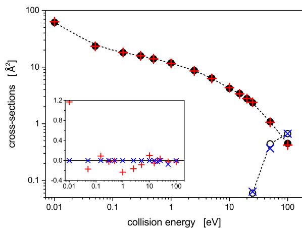
Figure 6. Comparison of type 1 momentum-transfer cross-sections and dissociation cross-sections as obtained for N_2^+(j=0,v=0)/He collisions via the MCSCF/avqz(spdf) method (full and open circles, respectively) and using artificial neural network (ANN) representations of the N_2^+/He potential energy surface (pluses and crosses, respectively). In the inset, deviations between the ANN and MCSCF/avqz(spdf) data (ANN–MCSCF) are depicted.
