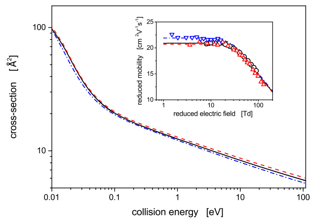
Figure 1. Type 1 momentum-transfer cross-sections calculated from selected experimental mobility data via the inverse-method (IM) approach: full line – IM cross-sections obtained from mobility data given in Ref. [40] (as reported in Ref. [43]), dashed line – IM cross-sections based on the mobilities of Ref. [41], and dash-dotted line – IM cross-sections based on Ref. [42]. In the inset, related experimental mobilities are provided for comparison (circles Ref. [40], up triangles Ref. [41], and down triangles Ref. [42]) together with their IM representations (using the same line patterns as in the main panel.)
