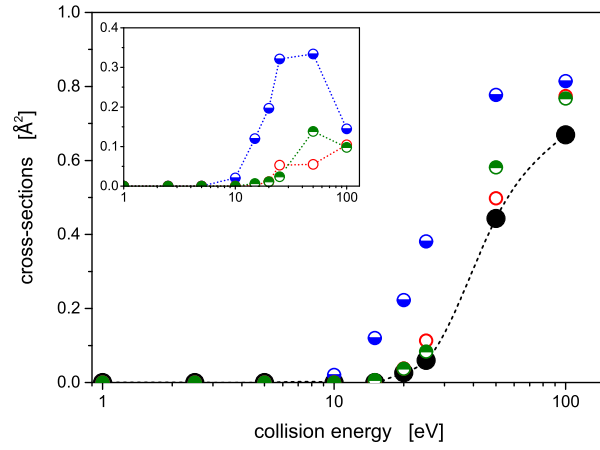
Figure 5. The same as in Fig. 2, but for the collision-induced dissociation cross-sections (Eq. (2)).
