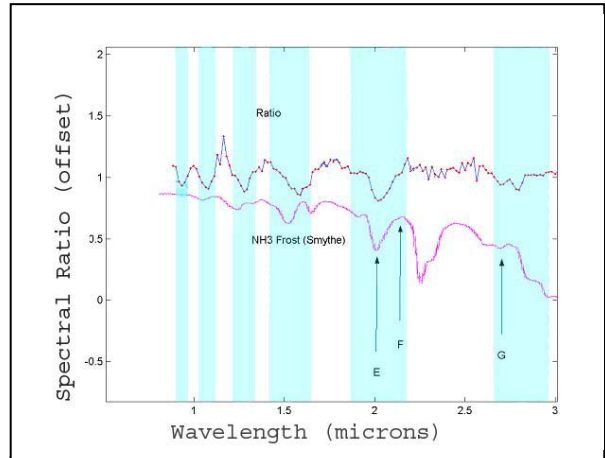
Fig4b. The ratio is divided by the normalized spectrum of the background to effect different amount of methane haze correction. This displays the NH 3 absorption features E=2.01 μm , F=2.13 μm , and G=2.69 μm.
