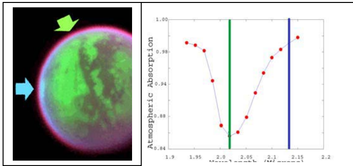
Fig 3. Left-RGB image of Fig 1. G (2.02 μm) is at the center of the methane window. B (2.13 μm) is at the band wing and shows the elevated cloud. R is 2.4 μm where CH 4 is completely opaque. Right- Titan's spectrum, 1.94-2.16 μm
