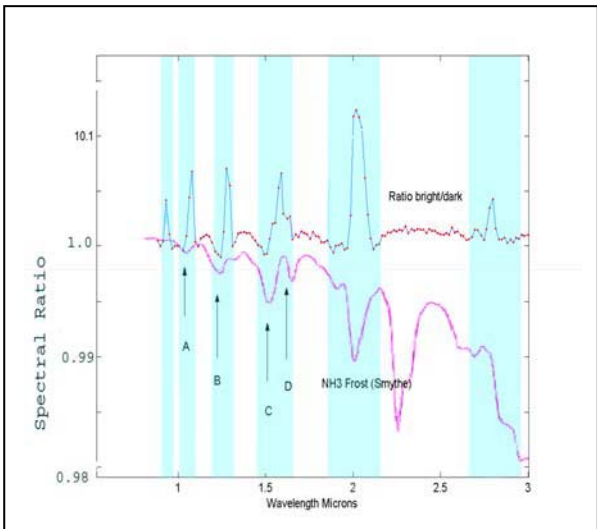
Fig 4 a. The NH 3 frost features are seen in the ratio at A=1.05 μm, B=1.24 μm, C=1.52 μm, and D=1.65 μm.
