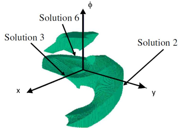
Fig. 31: Example of assembly mode changing trajectory of the 3-RPR parallel robot in joint space for \rho_1 = 15 .
