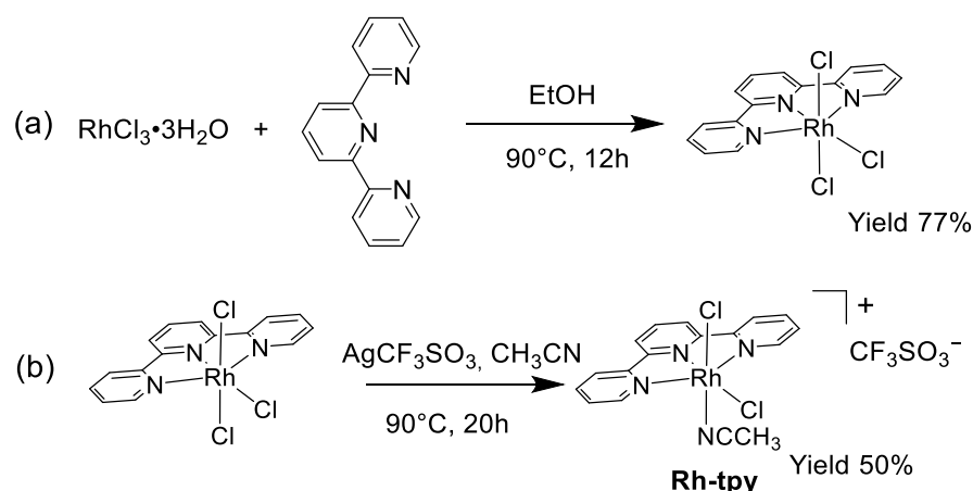
Scheme 3. Synthesis of the [\text{Rh}^{\text{III}}(\text{tpy})\text{Cl}_3] (a) and [\text{Rh}^{\text{III}}(\text{tpy})(\text{CH}_3\text{CN})\text{Cl}_2](\text{CF}_3\text{SO}_3) (b) ( Rh-tpy ) Complexes.
