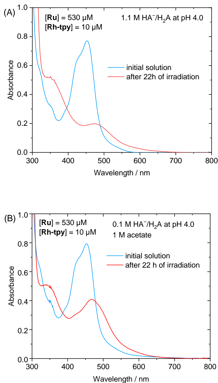
Figure 5. UV-vis absorption spectra of (A) Ru (530 μM) in aqueous solution containing NaHA/H 2 A (1.1 M) at pH 4.0 in presence of Rh-tpy (10 μM), (B) Ru (530 μM) in acetate buffer (1 M) at pH 4.0 containing NaHA/H 2 A (0.1 M) in presence of Rh-tpy (10 μM), initial solutions and after about 22 h of irradiation. Optical path = 1 mm.
