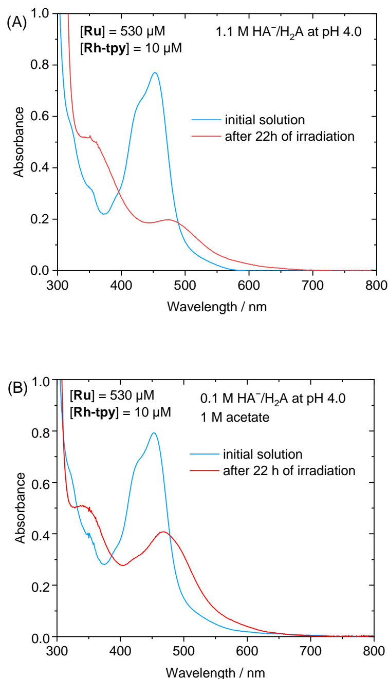
Figure 5. UV-vis absorption spectra of (A) Ru (530 \mu M ) in aqueous solution containing NaHA/ H_2A (1.1 M) at pH 4.0 in presence of Rh-tpy (10 \mu M ), (B) Ru (530 \mu M ) in acetate buffer (1 M) at pH 4.0 containing NaHA/ H_2A (0.1 M) in presence of Rh-tpy (10 \mu M ), initial solutions and after about 22 h of irradiation. Optical path = 1 mm.
