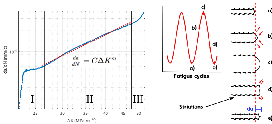
FIGURE 8 – Left : the 3 classical regimes of fatigue crack growth \frac{da}{dN} versus \Delta K from 5083 test : I threshold regime - II Paris regime - III fracture regime. Right : Mechanism of crack propagation by plasticity in Paris regime ; formation of striations
