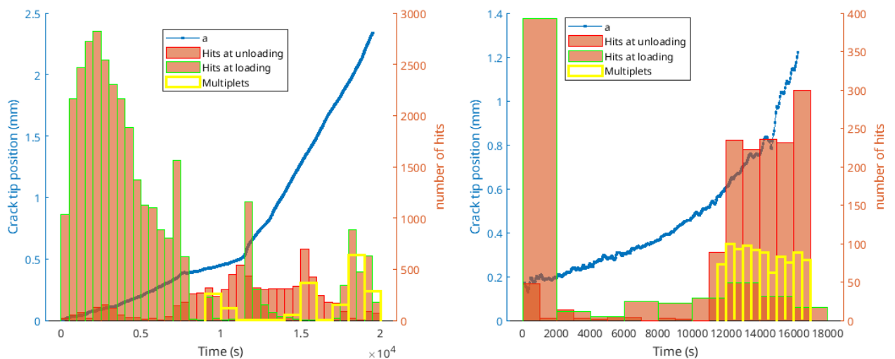
FIGURE 7 – Crack length versus time and number of AE signals recorded during loading, unloading, and number of signals belonging to an identified multiplet.
