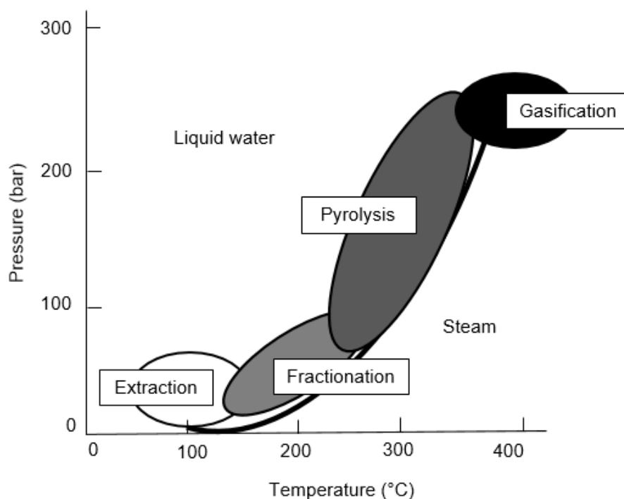
Figure 3: Temperature/pressure regimes for hydrothermal processing [22].
