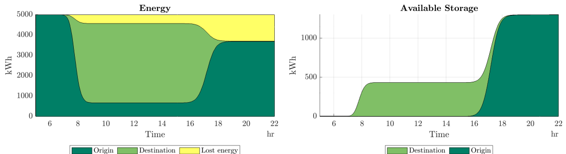
Figure 4: Energy consumption of EVs during one day.
