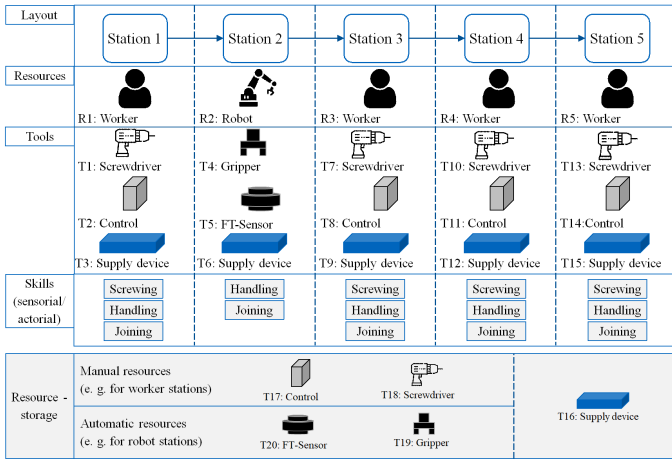
Fig. 8 Existing assembly line consisting of five stations
