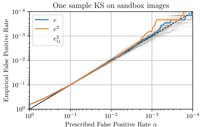
Fig. 1: Empirical false positive rate depending on theoretical false positive rate \alpha . Computed on 1M random images \mathbf{x} \sim \mathcal{U}_{\{0,255\}}^N . Black lines are the 64 KS(e_{ij}^2, \nu(0, \frac{1}{12})^2) without Bonferroni procedure and aggregation.
