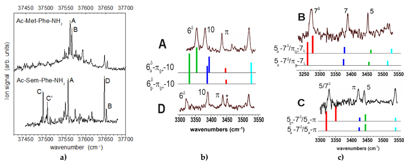
Figure 3: a) left panel : Near UV spectrum of the Ac-Sem-Phe-NH 2 molecule in the origin region of first \pi\pi^* transition of Phe, as obtained by mass-selected R2PI. Top : For comparison, the same spectrum for the related compound with Met, adapted from Ref. [19], is also shown. b) central and right panels : IR/UV double resonance spectra of conformers A-D (black traces), compared to the theoretical spectra (colored sticks) of selected best matching, low energy conformations (see Figure 2): A and D are assigned to folded 6^\delta - \pi -10 conformations; B and C to extended 5-7 o /5-7 forms. The IR experimental spectra (A-D) were recorded by probing the UV band bearing the same label in Fig. 1. The asterisk in spectrum D suggests a secondary contribution to the IR spectrum (see text for discussion). The color code of the stick spectra (green, red, blue and cyan bars) corresponds to NH stretches of the Sem, Phe residues and of the symmetric and antisymmetric C-terminal amide respectively.
