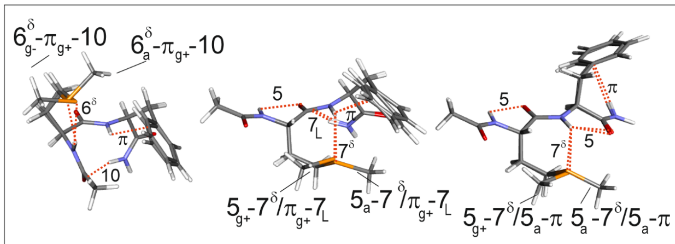
Figure 1: Typical low energy conformations of the folded (left), semi-extended (centre) and extended (right) conformational families of Ac-Sem-Phe-NH 2 , as obtained at the RI-B97D3(BJ-abc)/def2-TZVPPD level of theory (see text for terminology details). The folded and extended forms are shown with a gauche + and anti Phe side chain respectively (labelled by the second subscript), which corresponds to their most stable conformation. The family of semi-extended forms, illustrated here by the gauche + orientation, is much richer, since alternative backbone and side chain orientations can also be energetically competitive; also see text for the terminology used. Note here that for each conformation, the Sem side chain can exhibit two terminal orientations (labelled by the first subscript).
