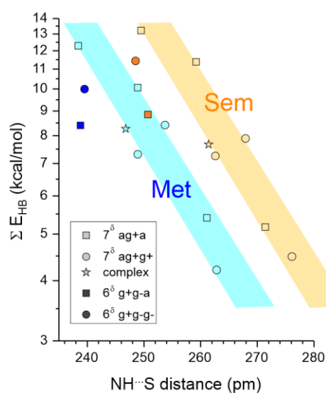
Figure 5: Semi-log plot of the stabilization energy \Sigma E_{HB} due to the NH \cdots S H-bonds (5SEE Table S3 and S4) against the NH \cdots S distance theoretically found for the 7^\delta and 6^\delta H-bonds (light and yellow symbols resp.) in the 5-7^\delta_{g+/g-}7_L , 5-7^\delta/5_a-\pi and 6^\delta-\pi_{g+}-10 backbone conformations of the Ac-Sem/Met-Phe-NH 2 dipeptides, with anti and gauche orientations of the Sem/Phe terminal dihedral \chi_3 (square and disk symbol resp.) together with the intermolecular MAA \cdots S/SeMe 2 complexes (stars). According to a previous NBO study of amide \cdots amide interactions,[29] points aligned on a same trend illustrate comparable H-bond efficiency of the geometrical approach and enable to assess frustration or enhancement of the H-bond by its environment (see details in text).
