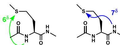
Scheme 1: Local side chain – backbone interactions of a Met side chain.
