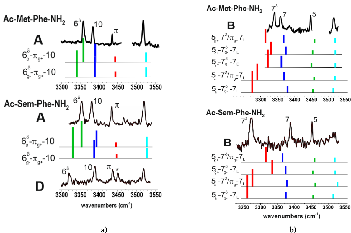
Figure 4: a) left panel : IR/UV double resonance spectra of folded conformers observed in the Sem-Phe and Met-Phe sequences, compared to the theoretical spectra (colored sticks) of selected best matching, low energy conformations. The comparison illustrates the similarities of the 6 δ H-bonds in these sequences; b) right panel : same pictures for the semi-extended conformers B, emphasizing the apparent differences in the 7 δ H-bonds between the two sequences. See text for assignment.
