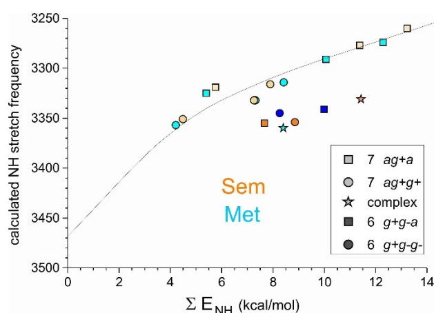
Figure 7 : Calculated NH stretch frequency (scaled harmonic frequencies) vs. the total stabilization energy (noted \Sigma E_{NH} ), taking into account all the interactions that contribute to the electron delocalization towards the \sigma^*_{NH} interaction, for the NH groups involved in a NH⋯Se/S interaction.
