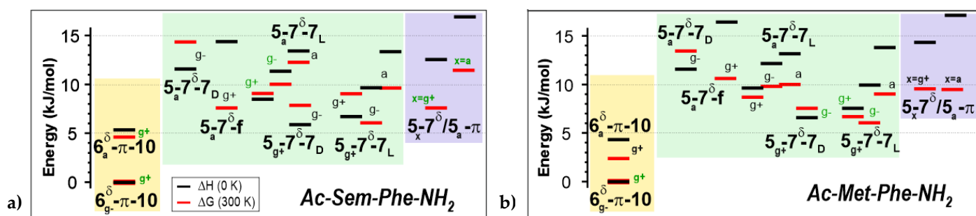
Figure 2: Conformational landscape of Sem-Phe ( left panel; a ) and Met-Phe ( right panel; b ) peptide chains, obtained at the RI-B97-D3(BJ-abc)/def2-TZVPPD level of theory. The 0 K \Delta H relative energies (resp. 300 K Gibbs energies, \Delta G ) are given as black (resp. red) lines. The conformation labels refer to the sequential status of the N-H bonds along the backbone (see text). The g^+/g^-/a subscripts of the folded and semi-extended conformations refer to the \chi_3 dihedral of the Sem/Met side chain; the labels associated to the bar of each conformation refer to Phe side chain \chi_1 orientation ( g^+/g^-/a ). In the extended conformation family, the x label refers to the Sem/Met side chain \chi_3 dihedral. Green labels indicate conformations, which are consistent with experimental observations.
