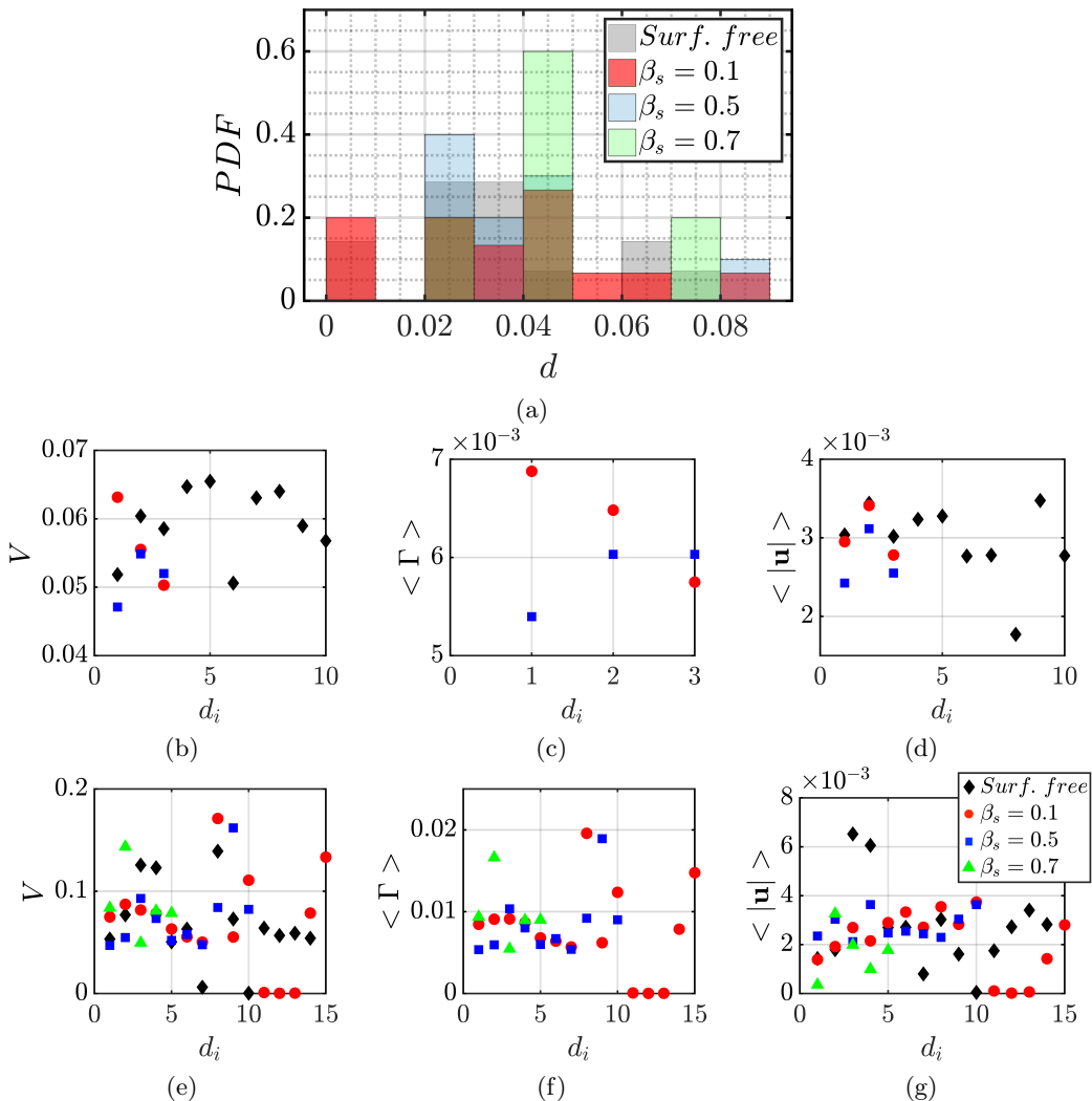
Figure 11: Metrics of splashing as a function of the elasticity parameter \beta_s . Panel (a) shows the probability density function (PDF) of the droplet size; droplet sizes are made dimensionless by the initial droplet diameter. Panels (b) – (d) and (e) – (g) show the volume, average surfactant concentration, and average velocity for every droplet at t = 15 , and t = 20 , respectively. All other parameters remain unchanged from figure 3.
