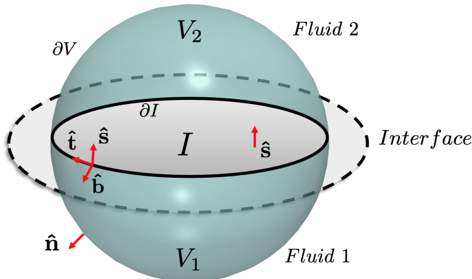
Figure 2: Schematic showing a volume V with a surface \partial V which encloses two fluids separated by an interface surface I . Here, the two smaller control volumes V_1 and V_2 refer to the control volume of each fluid. Local unit vectors to the interface are \hat{\mathbf{b}} , \hat{\mathbf{s}} and \hat{\mathbf{t}} ; \hat{\mathbf{n}} corresponds to the unit normal vector to the control volume \partial V , \hat{\mathbf{b}} is a vector tangent to I , but orthogonal to \partial I , and \hat{\mathbf{t}} is the unit tangent vector to the boundary curve \partial I .
