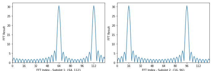
Fig. 5: The FFT result in sub-slot 1 (on the left) and 2 (on the right) for two symbols that are synchronized. The values of the symbols are 48 and 96, SF=7 , BW=125 kHz, and there are four sub-slots.
