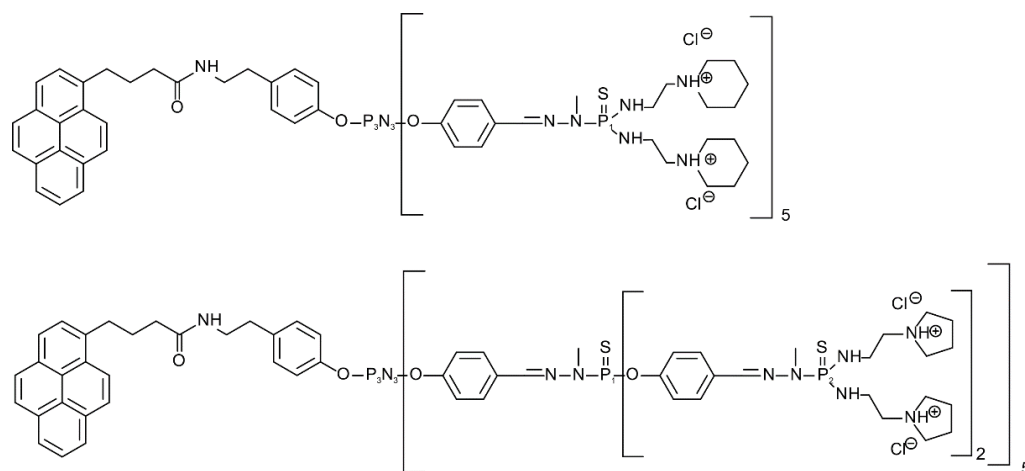
Figure 1. Structure of first-generation dendron, D1 ( top ); second-generation dendron, D2 ( bottom ).
