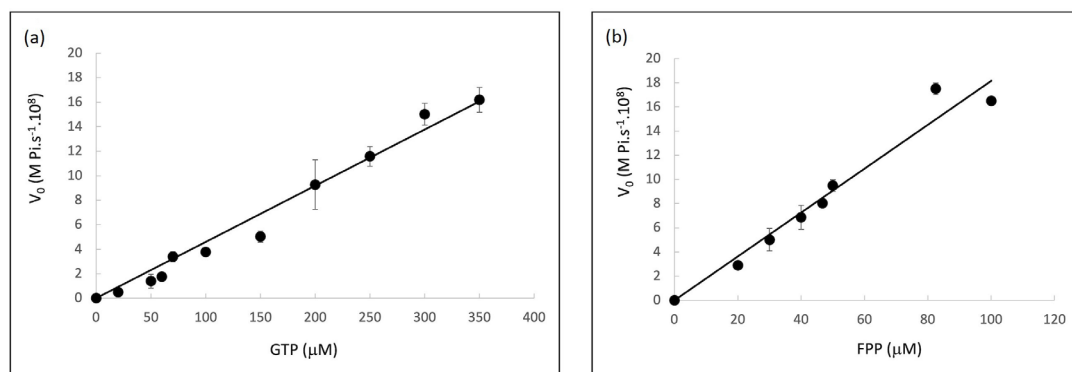
Fig. 7. Michaelis–Menten plots (initial rate V_0 in function of the substrate concentration) for GTP (a) and FPP (b). V_0 were measured with 16 and 3 \mu g \text{ ml}^{-1} of Cg1246-His for GTP and FPP, respectively, and expressed as Pi concentrations (M) released in the reaction medium, by second. Each value is the means \pm standard deviation of three independent experiments. For both GTP and FPP, values could not be fitted by an hyperbole and showed linear patterns. The slope of the lines (which represents k_{cat}/K_m ) were calculated from simple linear regression analysis using excel.
