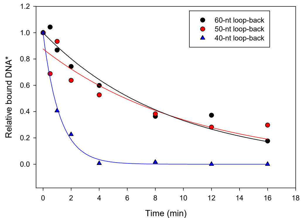
Figure 4. Dissociation rate constant ( k_{\text{off}} ) analysis of loop-back sequences derived from the E9-R5-12 P/T sequence. Loop-backs are described in Section 3 and shown in Table 1. Experiments were performed using nitrocellulose filter binding, as described in Section 2. * Values are relative to the value for the amount of loop-back DNA bound to E9 at time “0” (see Section 2), which was set to “1”.
