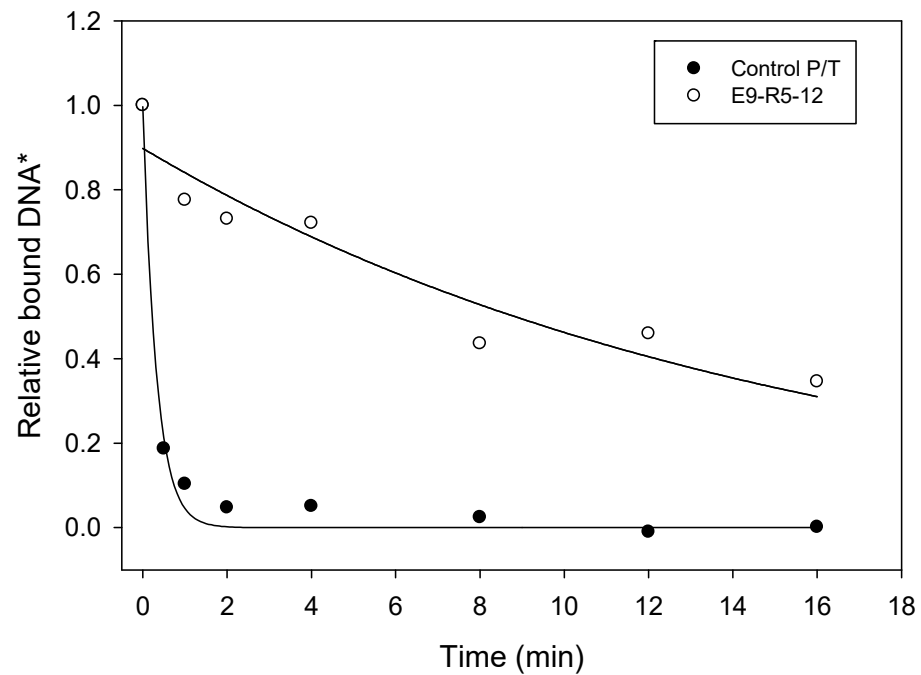
Figure 3. Dissociation rate constant ( k_{\text{off}} ) analysis of E9-R5-12 P/T sequence. Experiments were performed using nitrocellulose filter binding, as described in Section 2. * Values are relative to the value for the amount of DNA bound to E9 at time “0” (see Section 2), which was set to “1”. The sequences of the Control P/T and E9-R5-12 double-stranded DNA sequences are shown in Table 1.
