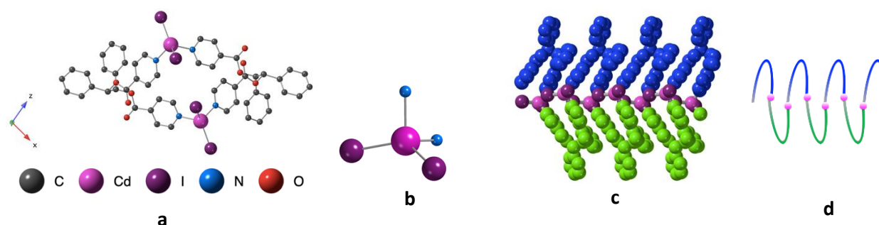
Figure 5: For L-CdI 2 a) portion of the X-ray structure of L-CdI 2 b) environment around the Cd 2+ cations c) the 1D helicoidal coordination polymer, projection in the xOz plane, and d) schematic representation of the helical 1D Structure. H atoms and chloroform solvent molecules are not represented for clarity.
