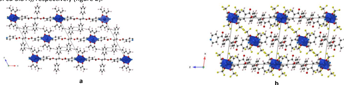
Figure 2 : Portion of the X-ray structure of L-Cu(acac) 2 (a) and L-Cu(hfac) 2 (b) showing the packing of consecutive chains in the xOz plane
