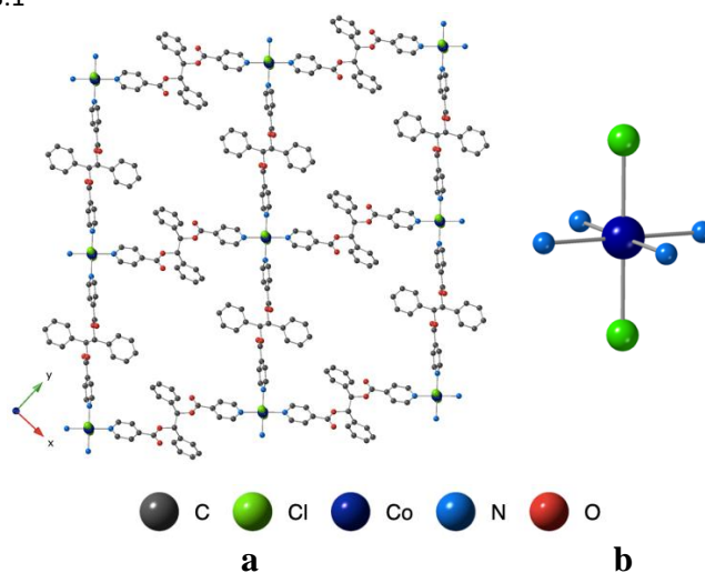
Figure 7: Portions of the X-ray structure of \text{L-CoCl}_2 showing the formation of grids between the connection of L with \text{CoCl}_2 metallaligands (left) and environment around the \text{Co}^{2+} cations. H atoms and chloroform solvent are not represented for clarity.
