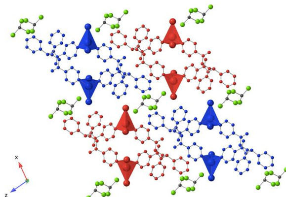
Figure 6: Portion of the X-ray structure of \text{L-CdI}_2 showing the packing of consecutive 1D zig-zag type networks in the xOz plane. H atoms are not represented for clarity.
