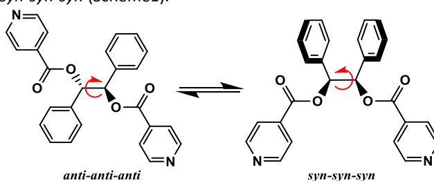
Scheme 1 : Two possible conformations for 1,2-Diphenylethane-1,2-diyl diisonicotinate ( L ).
