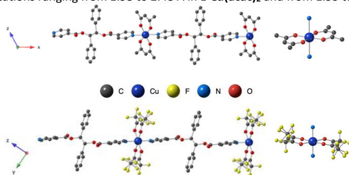
Figure 1 : Portion of the X-ray structure for L-Cu(acac) 2 (top left) and L-Cu(hfac) 2 (bottom left) showing the formation of the 1D neutral and linear coordination network resulting from the bridging of consecutive ligand L by Cu(acac) 2 (or Cu(hfac) 2 ) and environment around the Cu 2+ cations. H atoms are not presented for clarity.
