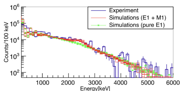
Fig. 4. Experimental spectrum of ^{254}\text{No} compared to simulated spectra with and without the M1 scissors mode. See the text for more details.
