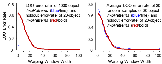
Figure 8. left : The LOO error-rate of the TwoPatterns 1000 dataset is a poor predictor of the holdout error on TwoPatterns 20 . right : In contrast, the average LOO error-rate of 20 random samples of TwoPatterns 20 dataset is an excellent predictor of the holdout error on TwoPatterns 20 .
