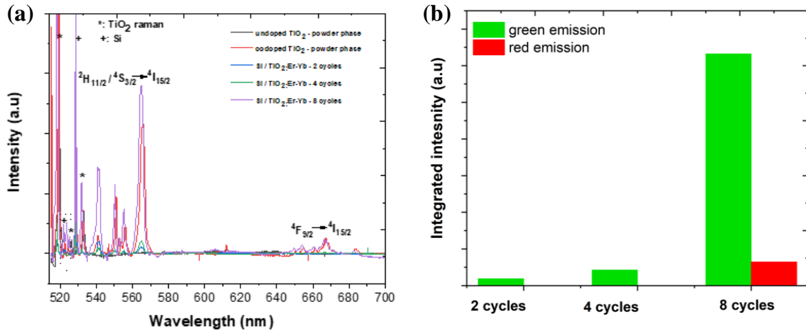
Fig. 3: (a) PL emission under excitation wavelength \lambda=514 nm of all the different samples from nanoparticles in powder phase to based thin film and (b) the corresponding integrated intensity of the peaks.
