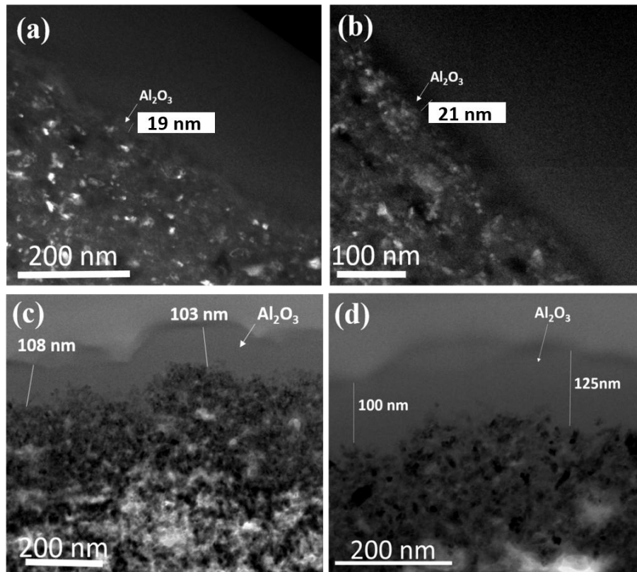
Fig. 5: HR-TEM images showing the thickness of (a, b) Si/TiO 2 :Er-Yb/62+FGA, (c, d) Si/TiO 2 :Er-Yb/620+FGA films.
