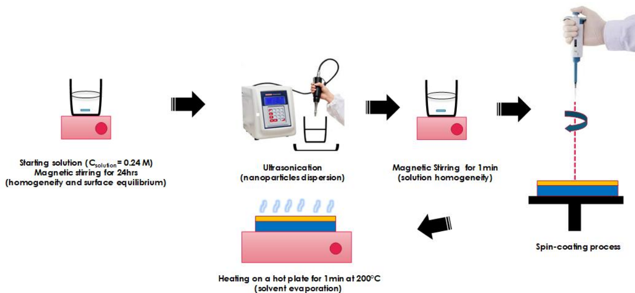
Fig. 1: Spin coating steps used.
