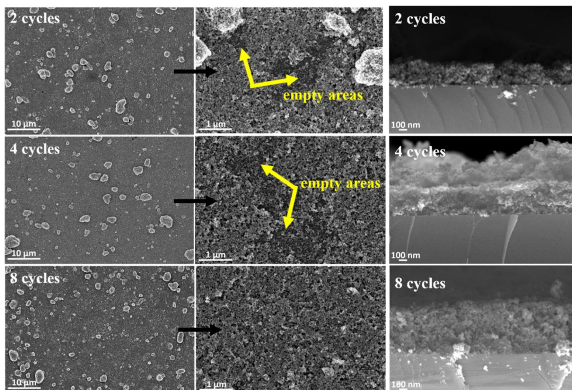
Fig. 2: SEM Top view images and cross sections of Si/TiO 2 :Er-Yb with different spin-coating cycle numbers (2, 4 and 8).
