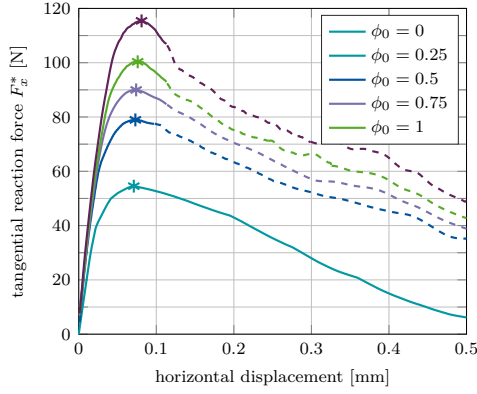
Figure 20: Tangential debonding with adhesive friction: Variation of the tangential force F_x^* as a function of the initial degree of osseointegration \phi_0 for the reference case. The maximum pull-out force F_x^{\max*} is marked with *.
