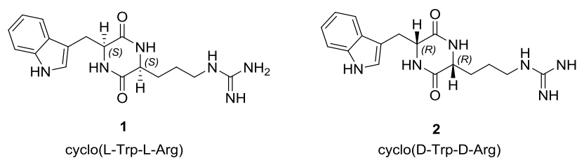
Figure 1. Proposed structures of CDP 2 ( 1 ) and CDP 3 ( 2 ) [8].
