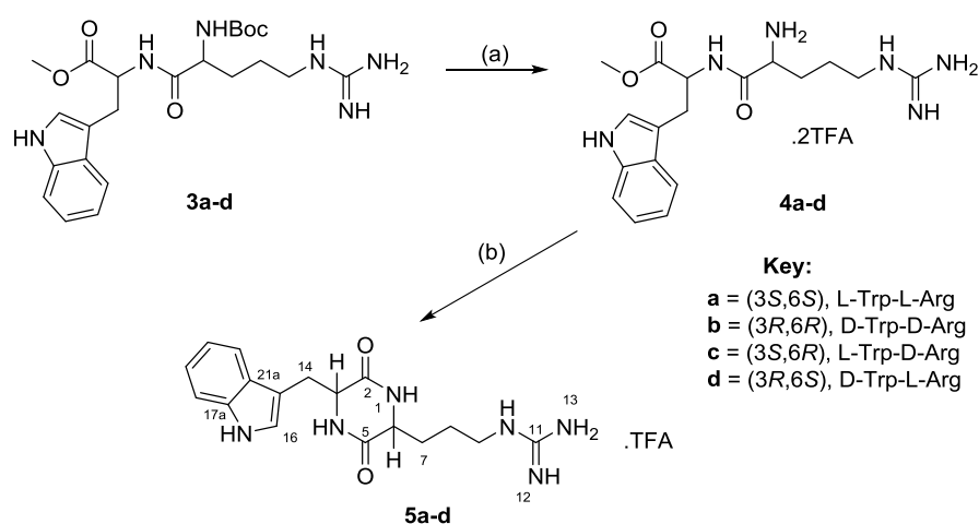
Scheme 1. General synthetic route for the synthesis of cyclo(Trp-Arg) stereoisomers.
