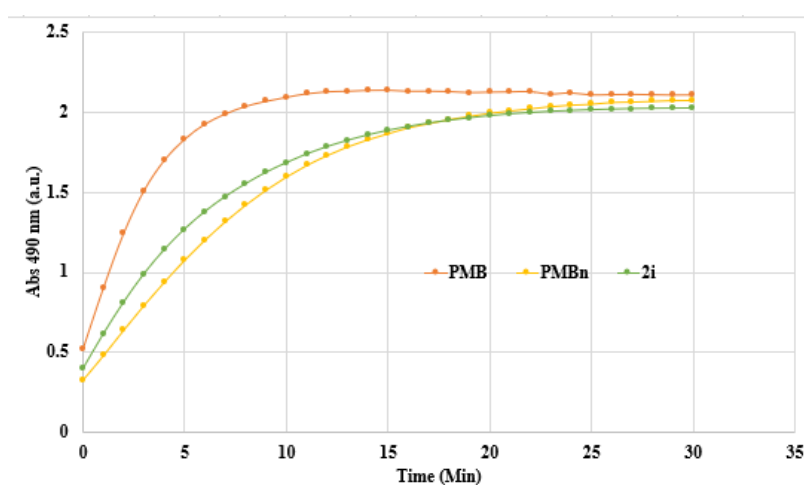
Figure 1. Nitrocefin hydrolysis kinetics in presence of compounds 2i at 18 \mu g/mL and compared to PMB and PMBn
