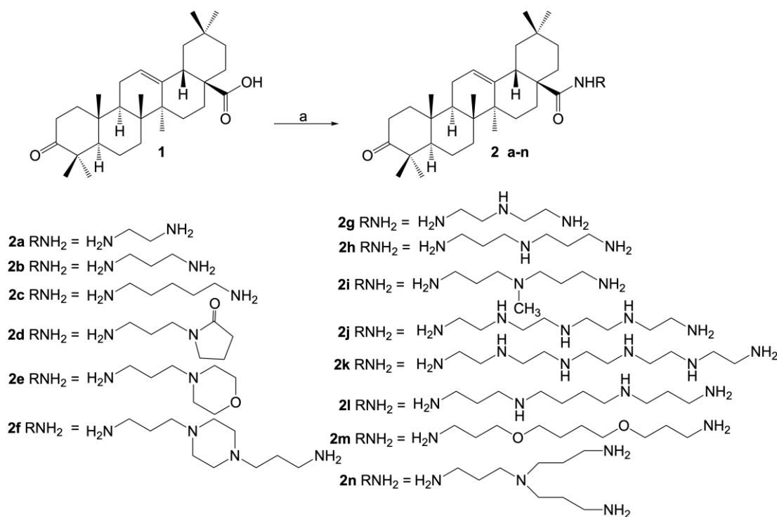
Scheme 1. Synthesis of oleanonic diamine and polyamine conjugates 2a-2n . Reagents and conditions: R-NH 2 , BOP, DIPEA, DCM, 20 °C, 12 h.
