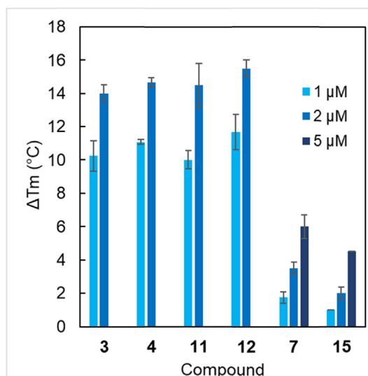
Fig. 3. FRET melting assays for compounds 1–16 with F21T G-quadruplex.
