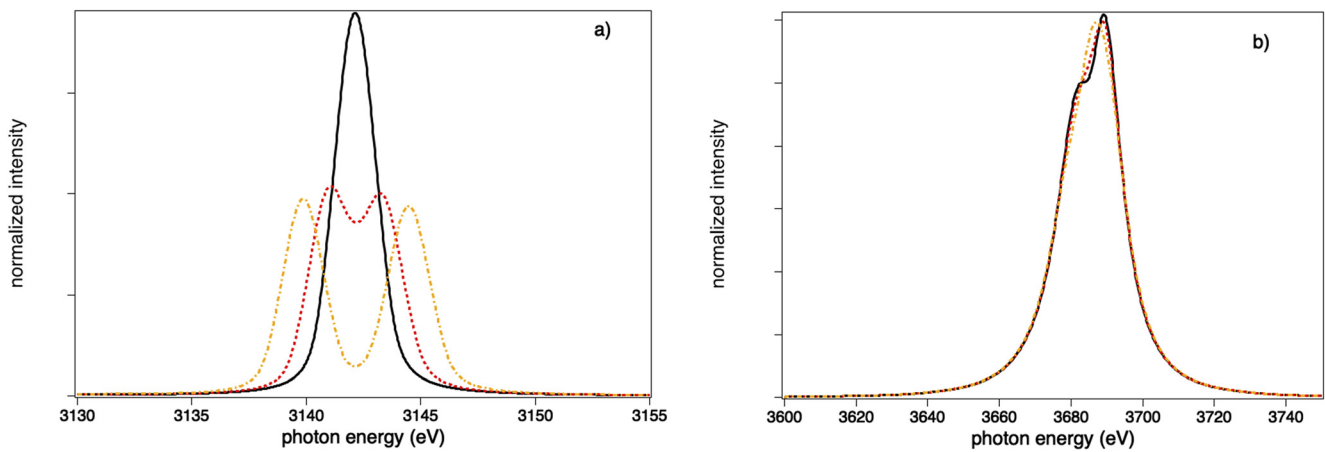
FIG. 10. Calculations of (a) Ar He- \alpha and (b) He- \beta SZ spectral lines for N_e = 5 \times 10^{23} \text{ cm}^{-3} , T_e = 2 keV, B = 0 (solid), B = 20 kT (dash), and B = 40 kT (dot-dash). A convolution with an instrumental resolution of E/\Delta E = 1800 is performed, and the observation is parallel to the magnetic field.
