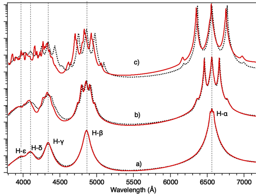
FIG. 1. Stark–Zeeman (SZ)-broadened Balmer-series lines for N_e = 10^{17} \text{ cm}^{-3} , T_e = 5 \text{ eV} , and B = (a) 100 T, (b) 500 T, and (c) 1 kT with (solid) and without (dashed) quadratic terms. The direction of observation is transverse to the B-field direction.
