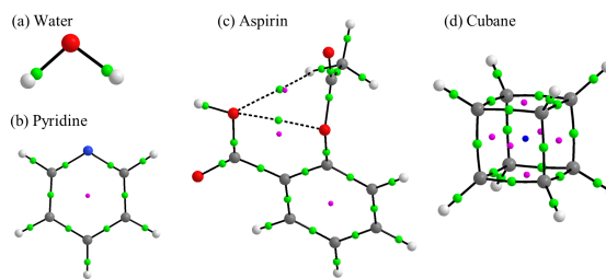
Fig. 1 Critical points of \rho(\mathbf{r}) and bond paths that connect them for (a) water, (b) pyridine, (c) aspirin, (d) cubane. CPs are shown as spheres. Bond critical points are colored in green, ring critical points are coloured in purple and cage critical points are colored in blue. Electronic structure calculations were performed at the PBE/def2-SVP level of theory, 20 and topological analysis was carried out by means of the AIMALL package. 21
