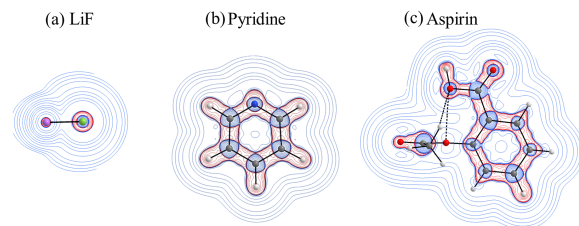
Fig. 2 Isocontours of \nabla^2\rho(\mathbf{r}) on planes containing selected bonds for: (a) LiF (ionic system), (b) pyridine (covalent system), and (c) aspirin (covalent system with non-covalent interactions). Negative Laplacian values are depicted in red, while positive ones are shown in blue. Electronic structure calculations were performed at the PBE/def2-SVP level of theory, 20 and topological analysis was made by means of AIMALL package 21
