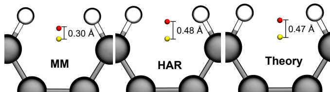
Fig. 5 Bond critical point (red) corresponding to the H \cdots H interaction in biphenyl. The distance to the ring critical point (yellow) is shown in angstroms for MM, HAR and solid-state DFT geometry optimization calculation. Data taken from reference 90
