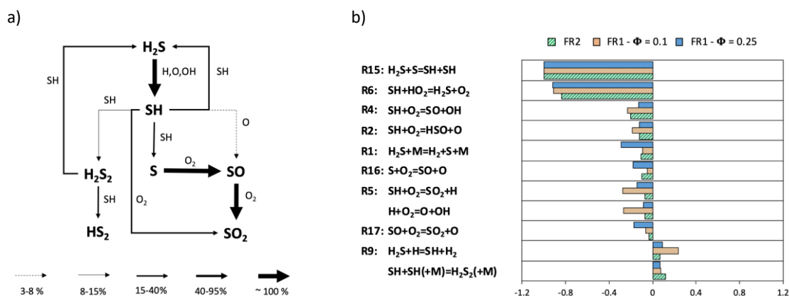
Figure 5. a) Sulfur flux analysis in the oxidation of 500 ppm H_2S in FR1. \Phi = 0.1 , \tau = 0.25 s. b) Sensitivity analysis to H_2S mass fraction (normalized with respect to the maximum value) in the 3 oxidation datasets for FR1 and FR2, in correspondence of H_2 peak. The reactor coordinate where 1% H_2S conversion was achieved was chosen for such evaluation.
