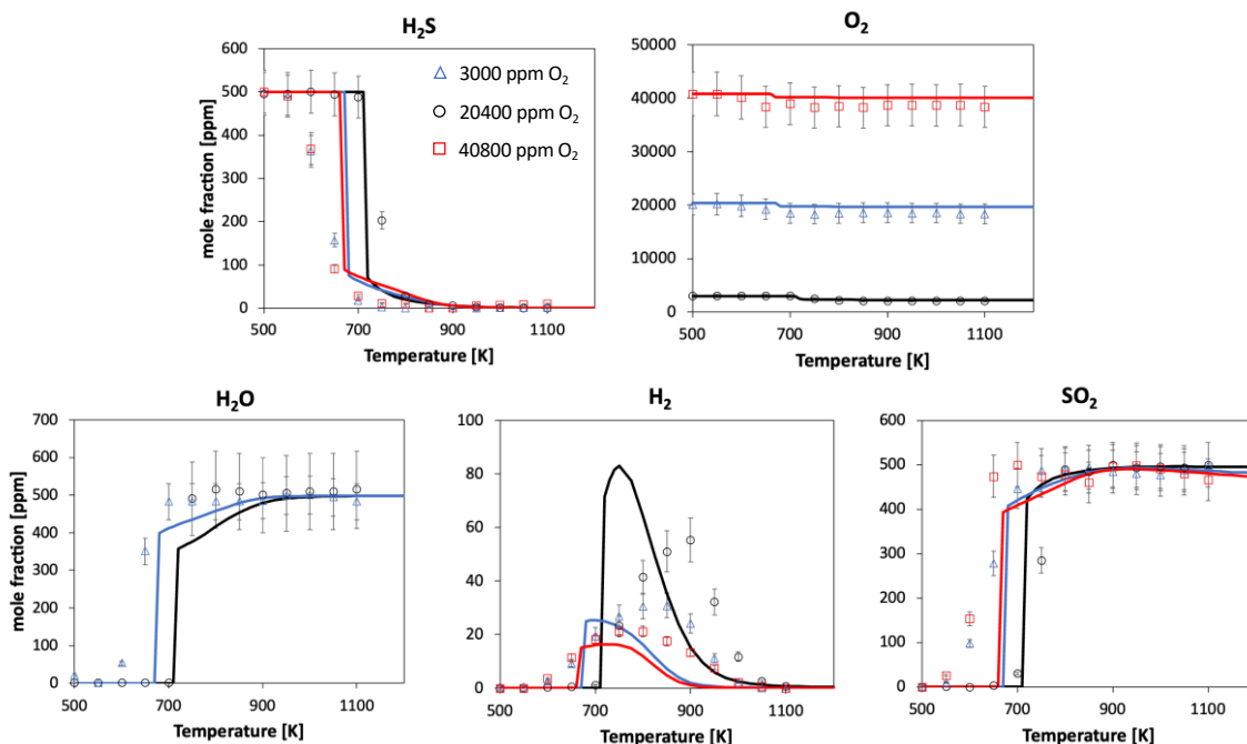
Figure 3. Oxidation of 500 ppm \text{H}_2\text{S} in a Jet-Stirred Reactor ( \tau = 2 s, P = 800 Torr) with variable amounts of \text{O}_2 . Experimental (symbols) and modeling (lines) results. Dashed lines indicate equilibrium mole fractions.
