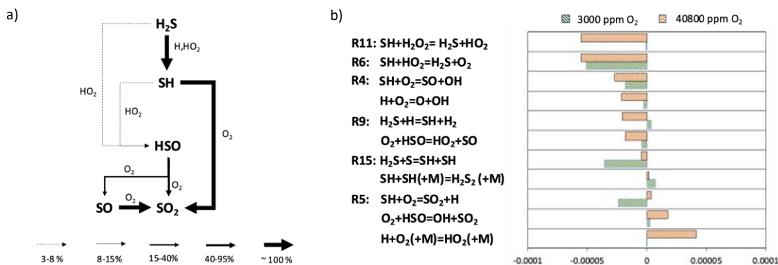
Figure 4. a) Sulfur flux analysis in the oxidation of 500 ppm \text{H}_2\text{S} with 40800 ppm \text{O}_2 in a JSR. T = 650 K. b) Sensitivity analysis to \text{H}_2\text{S} mass fraction with 3000 ppm \text{O}_2 ( T = 700 K) and 40800 ppm \text{O}_2 ( T = 650 K), respectively. \tau = 2 s. P = 800 Torr.
