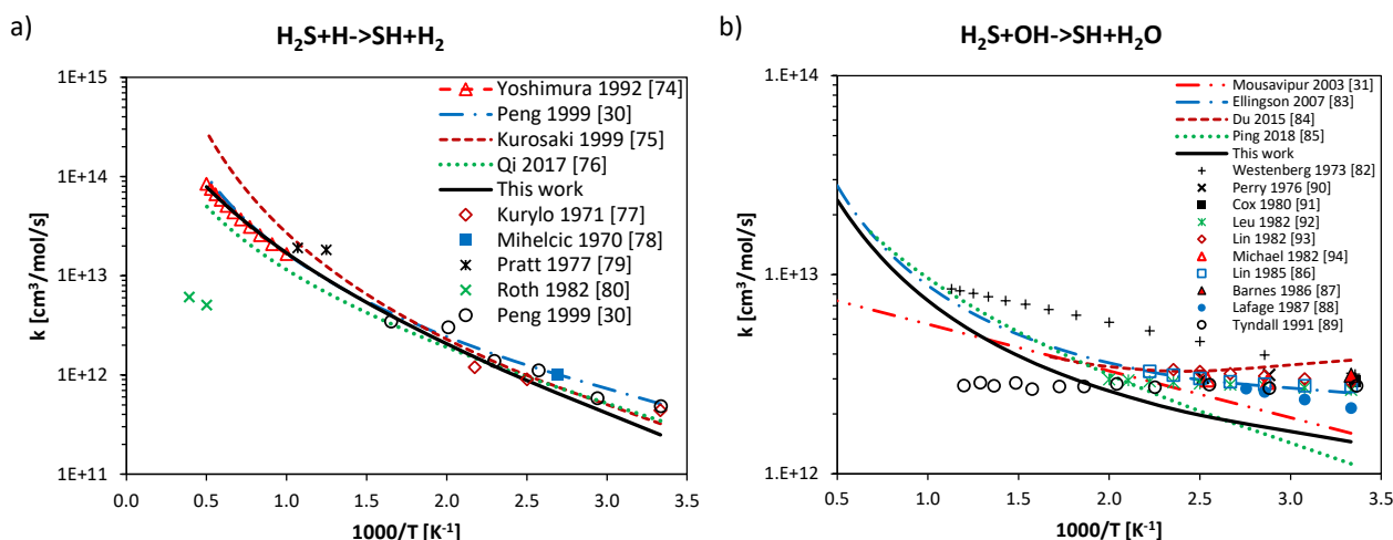
Figure 3. Computed rate constants for the H-atom abstraction reactions by a) H and b) OH from \text{H}_2\text{S} in comparison with the available theoretical [30,31,77-79,86-88] and experimental [30,80-83,85,89-97] literature estimates.
