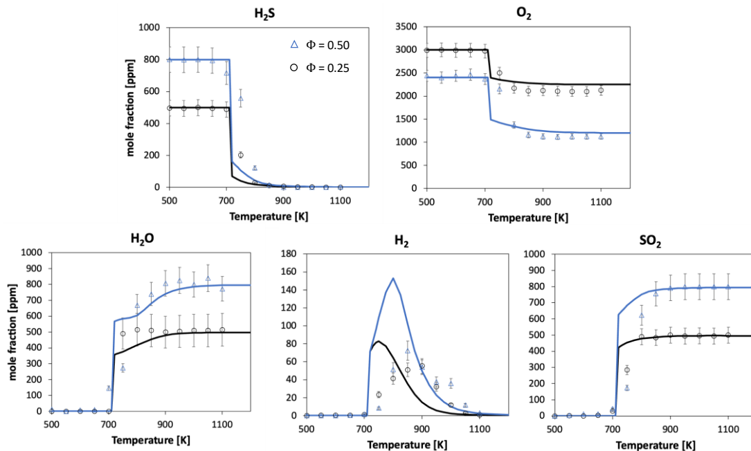
Figure 2. Oxidation of 500 ppm ( \Phi = 0.25 ) and 800 ppm ( \Phi = 0.50 ) \text{H}_2\text{S} in a Jet-Stirred Reactor ( \tau = 2 s, P = 800 Torr). Experimental (symbols) and modeling (lines) results.
