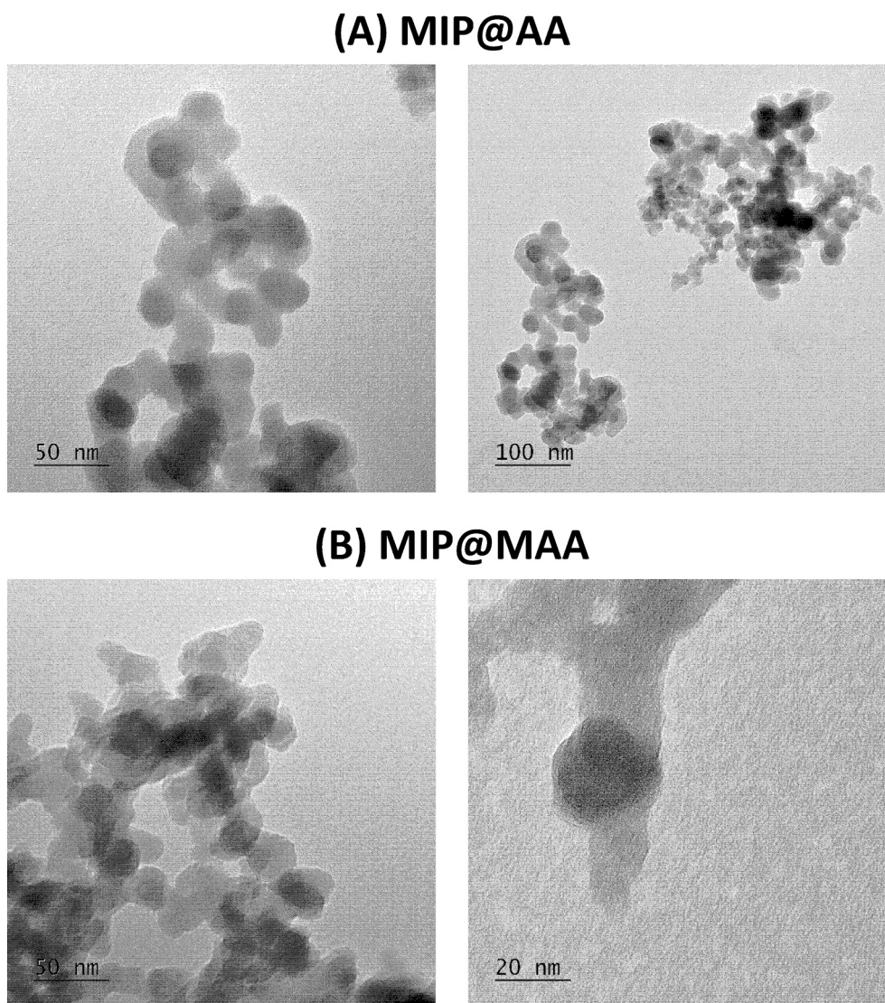
Fig. 4. TEM images MIP@AA (A) and MIP@MAA (B) at two magnifications.
