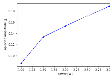
Fig. 13. Experiment results: impact of power on Laplacian peak-to-peak amplitude. Amplitude is measured for a spot at 6.2 mm from the crack. We see an increase of the response following the increase of power.
