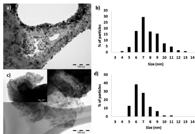
Fig. 4 TEM micrograph of \text{CuO}_x NPs@ \text{Fe}_3\text{O}_4 (a) and its particle size distribution graphic (b); TEM micrograph of \text{CuO}_x - \text{Fe}_3\text{O}_4 NPs@graphene (c) and its particle size distribution graphic (d). Reproduced from 30d with permission of Elsevier and Copyright Clearance Center (license number: 5160240128897) 2017.
