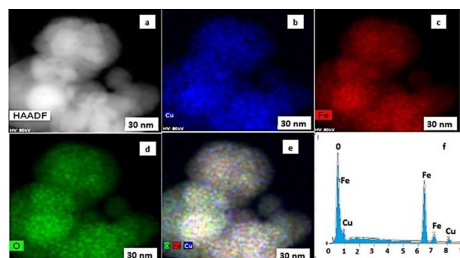
Fig. 23 HAADF-STEM images of Cu-maghemite nanocatalyst; a) HAADF image; b) Distribution of Cu by HAADF; c) Distribution of Fe by HAADF; d) Distribution of O by HAADF; e) Distribution of Cu, Fe, and O together by HAADF; f) EDS spectrum indicating the presence of Cu. Reprinted from 128 with permission of John Wiley and Sons and Copyright Clearance Center (license number: 5160250578857) 2015.
