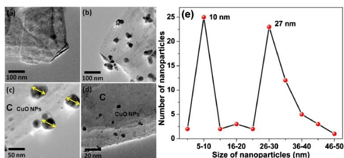
Fig. 15 TEM micrographs (a) Carbon nanopowder and (b, c and d) CuO NPs@Carbon nanopowder, and (e) size distribution histogram of CuO NPs. Reproduced from 76 with permission of Elsevier and Copyright Clearance Center (license number: 5160200537079) 2017.
