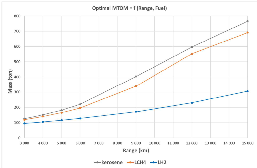
Fig 4. Optimal MTOM for different ranges and types of fuel
