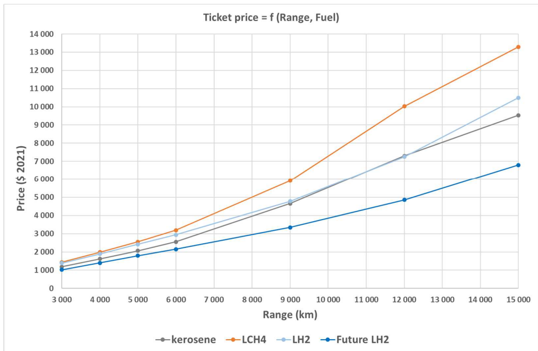
Fig 5. Ticket price associated to optimal MTOM for different ranges and types of fuel
