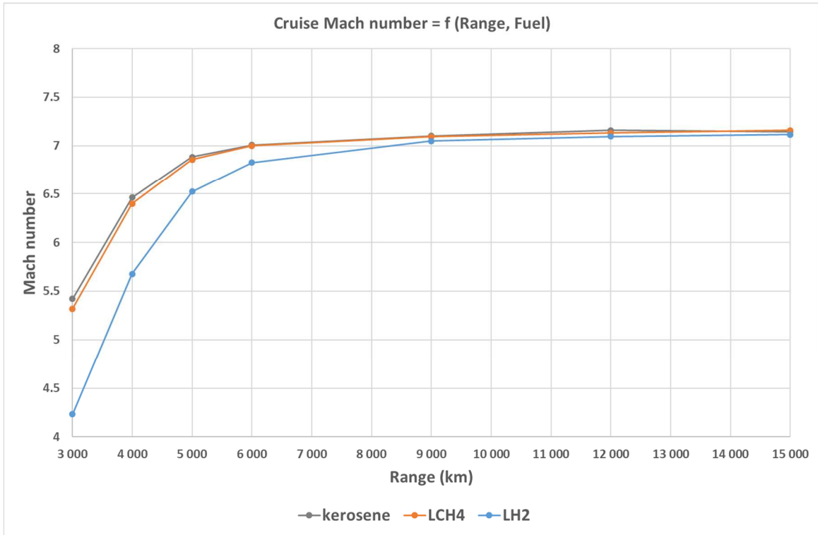
Fig 6. Cruise Mach number associated to optimal MTOM for different ranges and types of fuel
