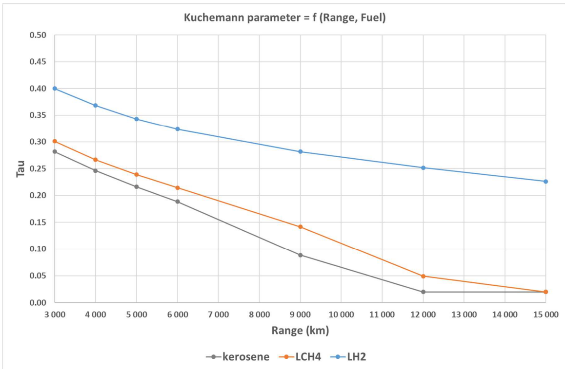
Fig 7. Kuchemann parameter associated to optimal MTOM for different ranges and types of fuel
