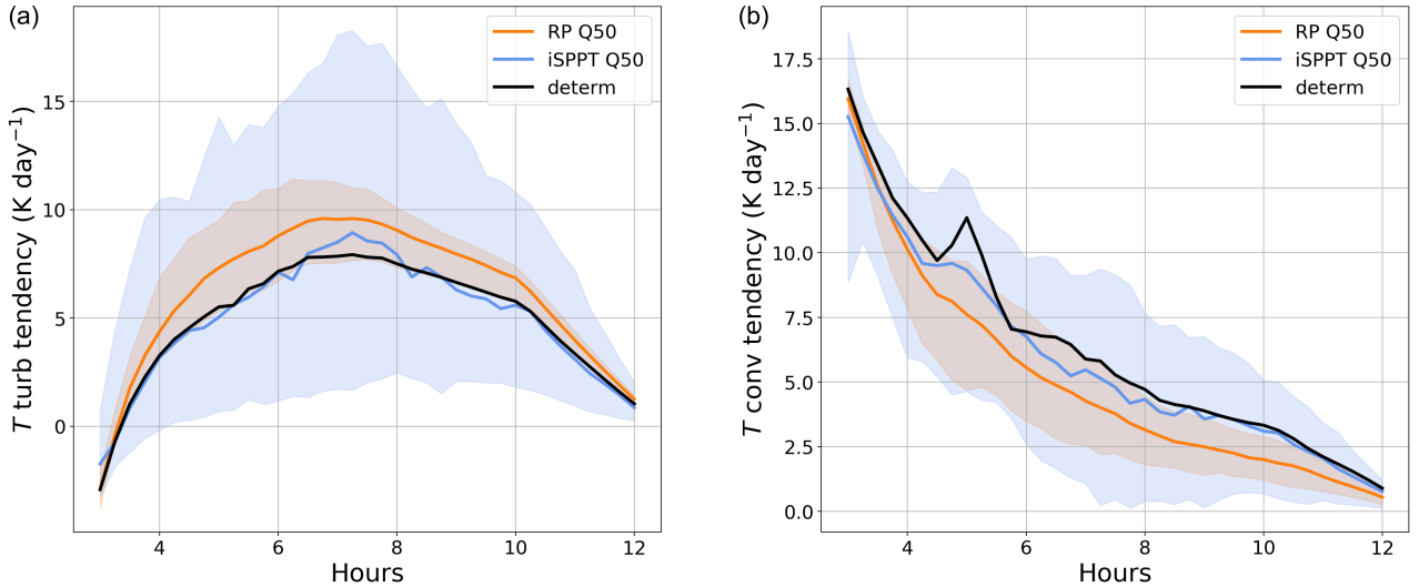
Figure 6: Time evolutions of the RP and iSPPT ensemble distributions of instantaneous temperature tendencies from (a) turbulence and (b) convection at 270 m, i.e., in the lower CBL.
