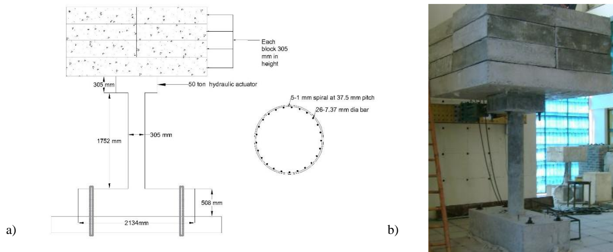
Figure 1: a. Geometry and b. Experimental test setup of the numerical model
