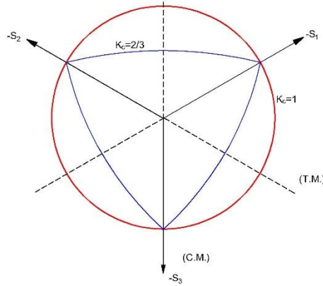
Figure 2: Yield Surface in deviatoric plane
