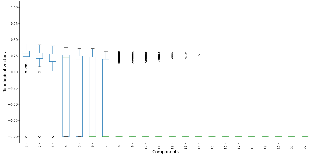
FIG. S28. Boxplots of the topological vectors in homological dimension H_2 for data in C_6 .
