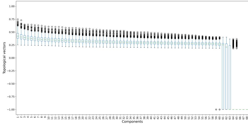
FIG. S20. Boxplots of the topological vectors in homological dimension H_0 for data in C_4 .
