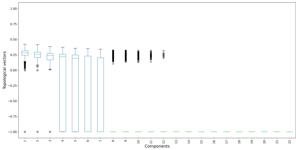
FIG. S25. Boxplots of the topological vectors in homological dimension H_2 for data in C_5 .
