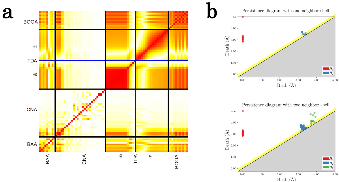
FIG. 5. (a) Empirical correlation matrix (absolute value) between several descriptor families: BAA, CNA, TDA, and BOOA. Low values are white, high values are red. We distinguish between the descriptors by black lines, and between levels of homology with a blue line ( H_0 and H_1 ). (b) PDs of a local atomic structure with one and two neighbor shells. The yellow line corresponds to a threshold computed with the subsampling approach to remove noises.
