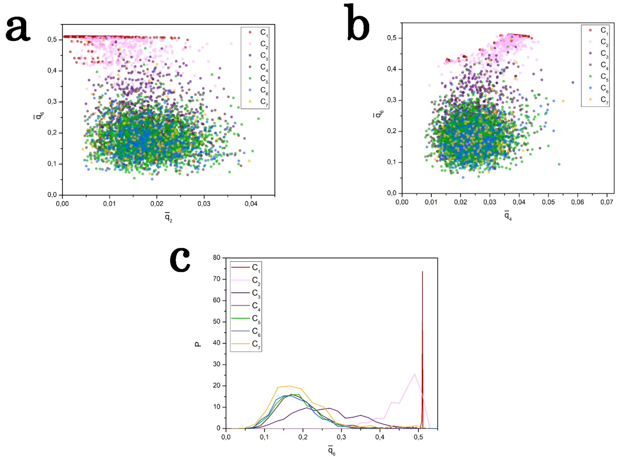
FIG. S33. (a) \bar{q}_2 - \bar{q}_6 -plane, (b) \bar{q}_4 - \bar{q}_6 -plane and (c) probability distributions of \bar{q}_6 , for the structures in the trained model.
