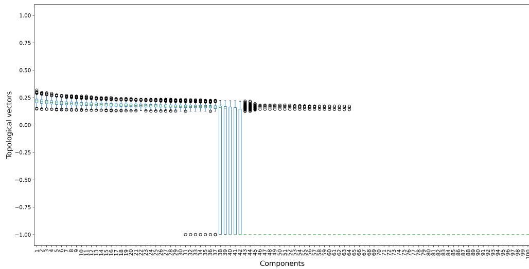
FIG. S21. Boxplots of the topological vectors in homological dimension H_1 for data in C_4 .
