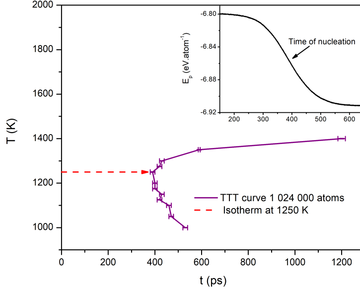
FIG. 1. Time-temperature-transformation curve with 1 024 000 atoms in a temperature range near the nose, which was obtained over 5 independent runs for each temperature . Inset: evolution of the potential energy as a function of time along a nucleation process. See more details in [21].
