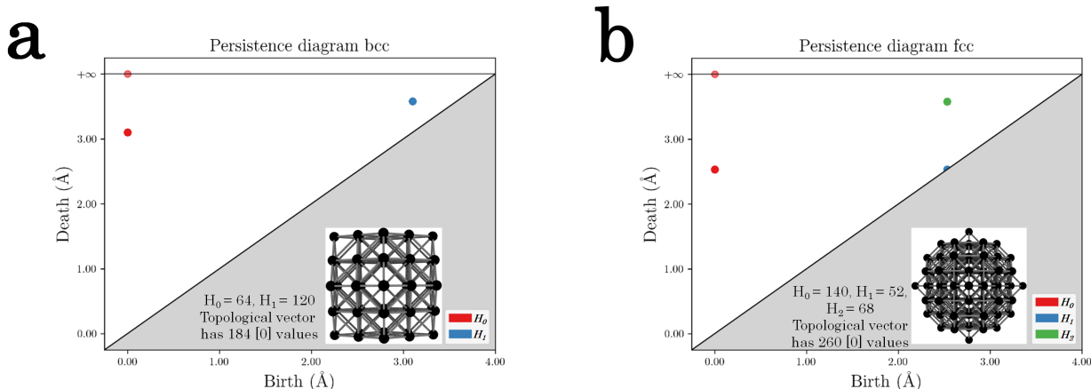
FIG. 4. (a) Zr atoms on a bcc lattice and the corresponding PD. (b) Zr atoms on a fcc lattice and the corresponding PD. The homological dimensions H_0 , H_1 , and H_2 are depicted in red, blue, and green respectively. As these structures are on periodic lattices, all topological features of the filtration from a specific homological dimension have the same pair (birth, death).
