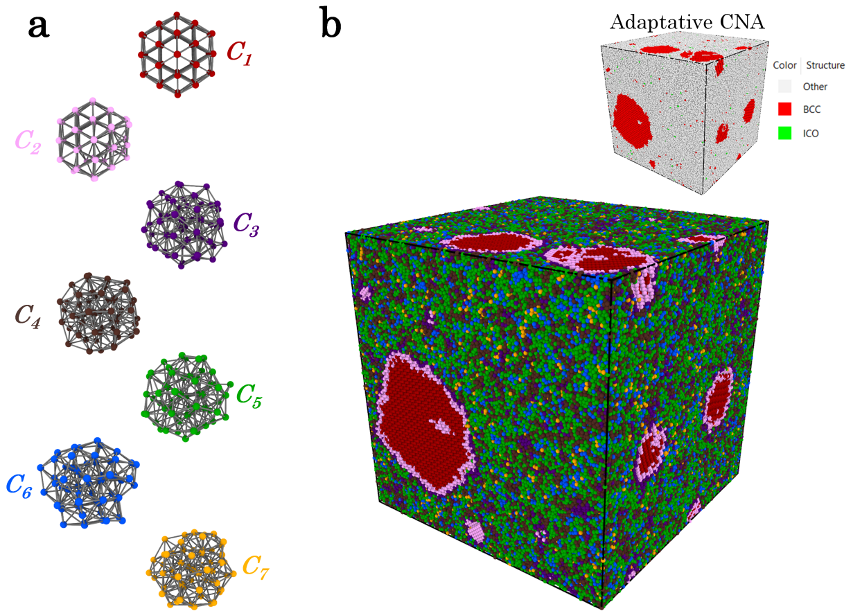
FIG. 7. (a) Representation in the real space of the local structures assigned to each cluster C_i . (b) Snapshot of the one million atoms in the simulation box after the clustering in the descriptor space. In the inset, the classification obtained from an adaptative CNA method is depicted.
