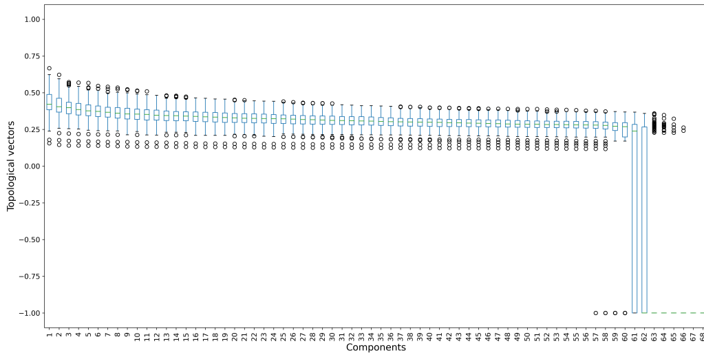
FIG. S29. Boxplots of the topological vectors in homological dimension H_0 for data in C_7 .
