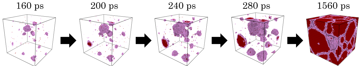
FIG. 9. Snapshots of Zr's configurations along nucleation at the nose of the TTT at T = 1250 K. The local structures in the clusters C_1 and C_2 identified as carrying the crystalline periodicity are depicted through their central particle in red and pink, respectively.
