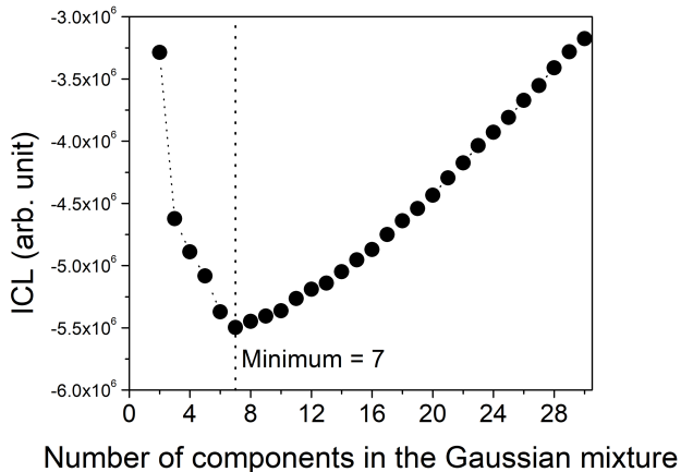
FIG. 6. ICL criterion on the training set. Its minimum corresponds to the maximum likelihood, which leads to the optimal number of clusters to build the model.
