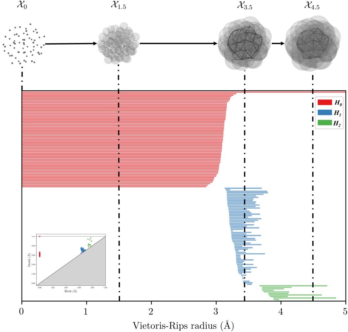
FIG. 3. Schematic snapshots of the Vietoris-Rips complexes filtration (\mathcal{X}_t)_{t \geq 0} applied to a local structure with two neighbor shells. The barcode below encodes the persistence of each topological feature by a line starting at its birth (the radius where its appear) and finishing at its death (the radius where it disappears). The colors correspond to the homological dimension (red, blue and green for H_0 , H_1 , and H_2 respectively) of each topological feature. The insert represents the corresponding PD where each point corresponds to a line, and thus its associated topological feature with coordinates (birth, death).
