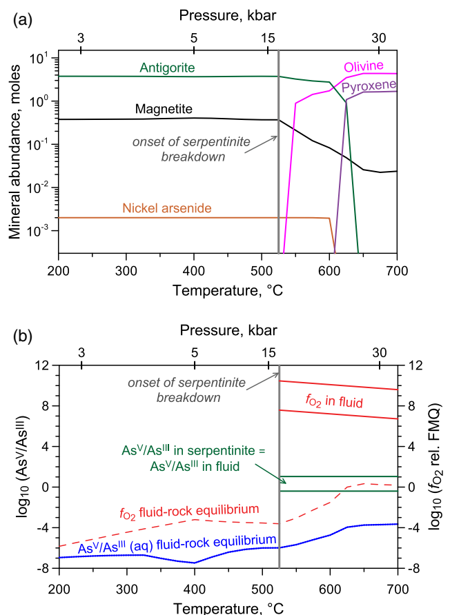
Figure 3 Thermodynamic simulations of serpentinitisation in the system harzburgite-sediment-aqueous fluid (starting mass ratios 10:1:10, respectively), along the T-P subduction path from Guillot et al. (2008). (a) Equilibrium relative abundances of key minerals. (b) Predicted As V /As III species ratio in the aqueous fluid (dotted blue) and f O 2 (dashed red) assuming bulk system equilibrium, as compared to the range of f O 2 in the fluid (lower and higher bounds, solid red) corresponding to the range of As V /As III ratios measured in serpentinite (solid green).
