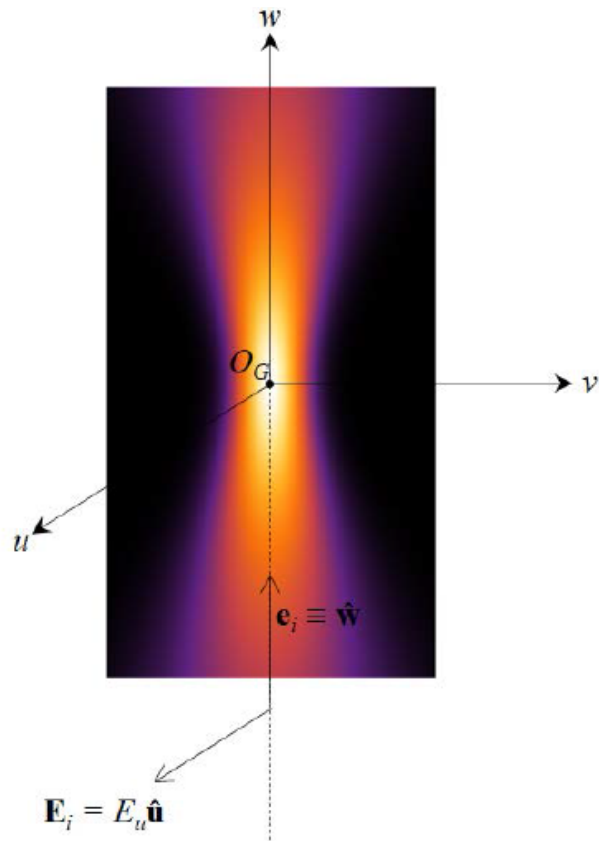
Fig. 2. Geometry and coordinate system for the illuminating beam. The beam is assumed to propagate along the w axis, with the v axis parallel to the z axis of Fig. 1. The electric field vibrates along the u axis.
