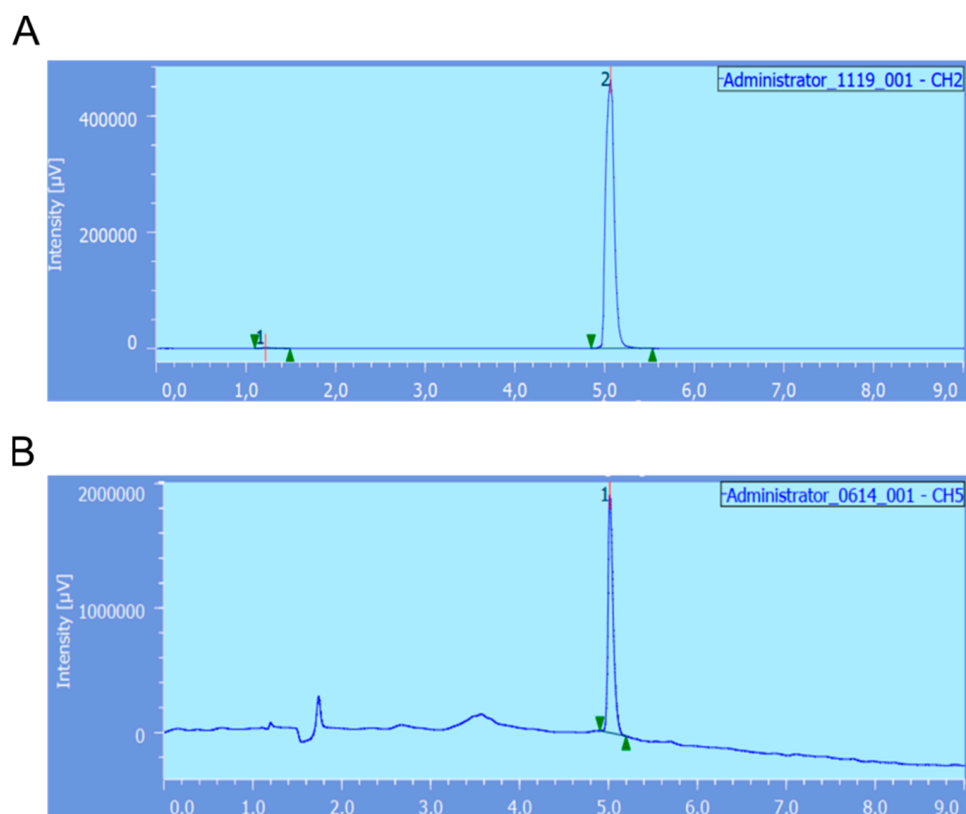
Figure 4. (A) radio-HPLC trace of [ ^{68}\text{Ga} ]Ga-RM2 obtained after direct radiolabeling of the kit developed in this study. Chemical identity was checked using [ ^{\text{nat}}\text{Ga} ]Ga-RM2 (UV-HPLC trace (B)).
