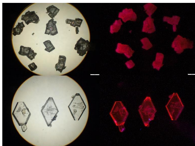
Figure 1. Optical microscopy pictures of crystals of \text{Cs}_3[\text{Eu}(\text{DPA})_3] \cdot 8\text{H}_2\text{O} ( 1 , bottom) and \text{Na}_3[\text{Eu}(\text{DPA})_3] \cdot 15\text{H}_2\text{O} ( 2 , top) under white (left) and UV (right) light irradiation.
