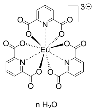
Chart 1. Compounds discussed in this article.
