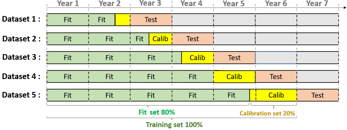
Figure 2: Sequential cross-validation scheme: testing conformal prediction on a cumulative time window.
