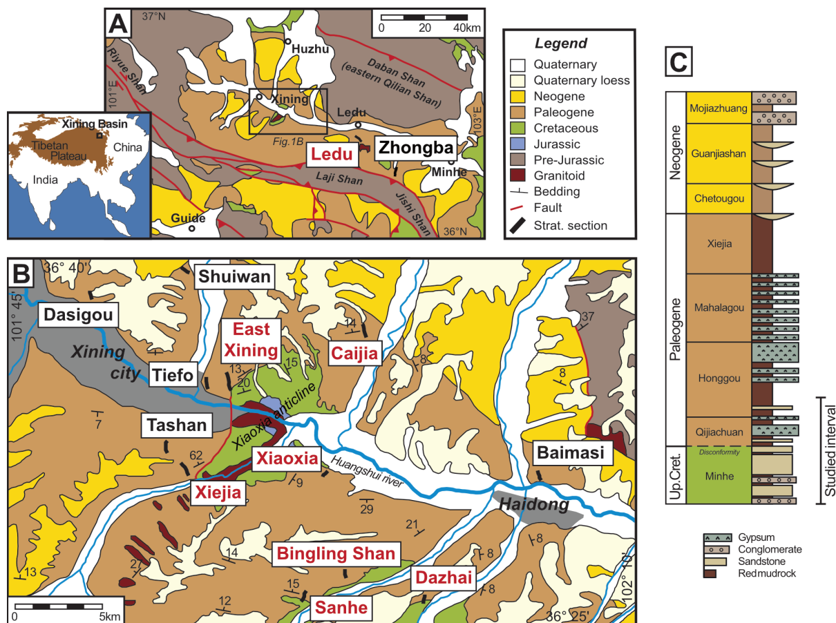
Fig. 1. A) Geological map of the Xining Basin (modified from Fan et al., 2019) showing the location of the studied Ledu section. Inset map shows the location of the Xining Basin. B) Detailed geological map (modified from BGMRQP, 1965 and QBGM, 1985) showing the section locations near Xining city. Sections used in this study are indicated in red. C) Generalized lithostratigraphic column of the Xining Basin (based on QBGM, 1985; Horton et al., 2004; Fang et al., 2019).
