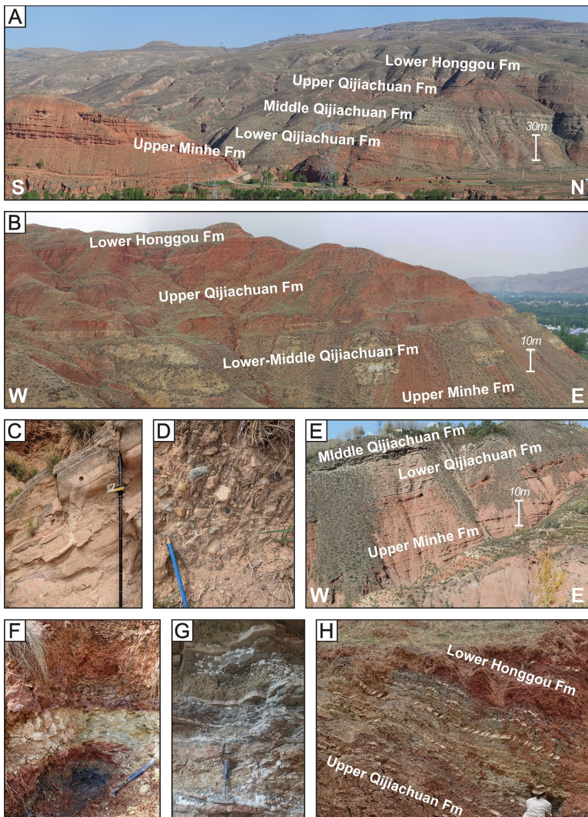
Fig. 3. Pictures of the studied sections and lithofacies. A) Overview of the Sanhe section. B) Overview of the Dazhai section. C) Sandstone of the Minhe Formation at the -150 meter-level
