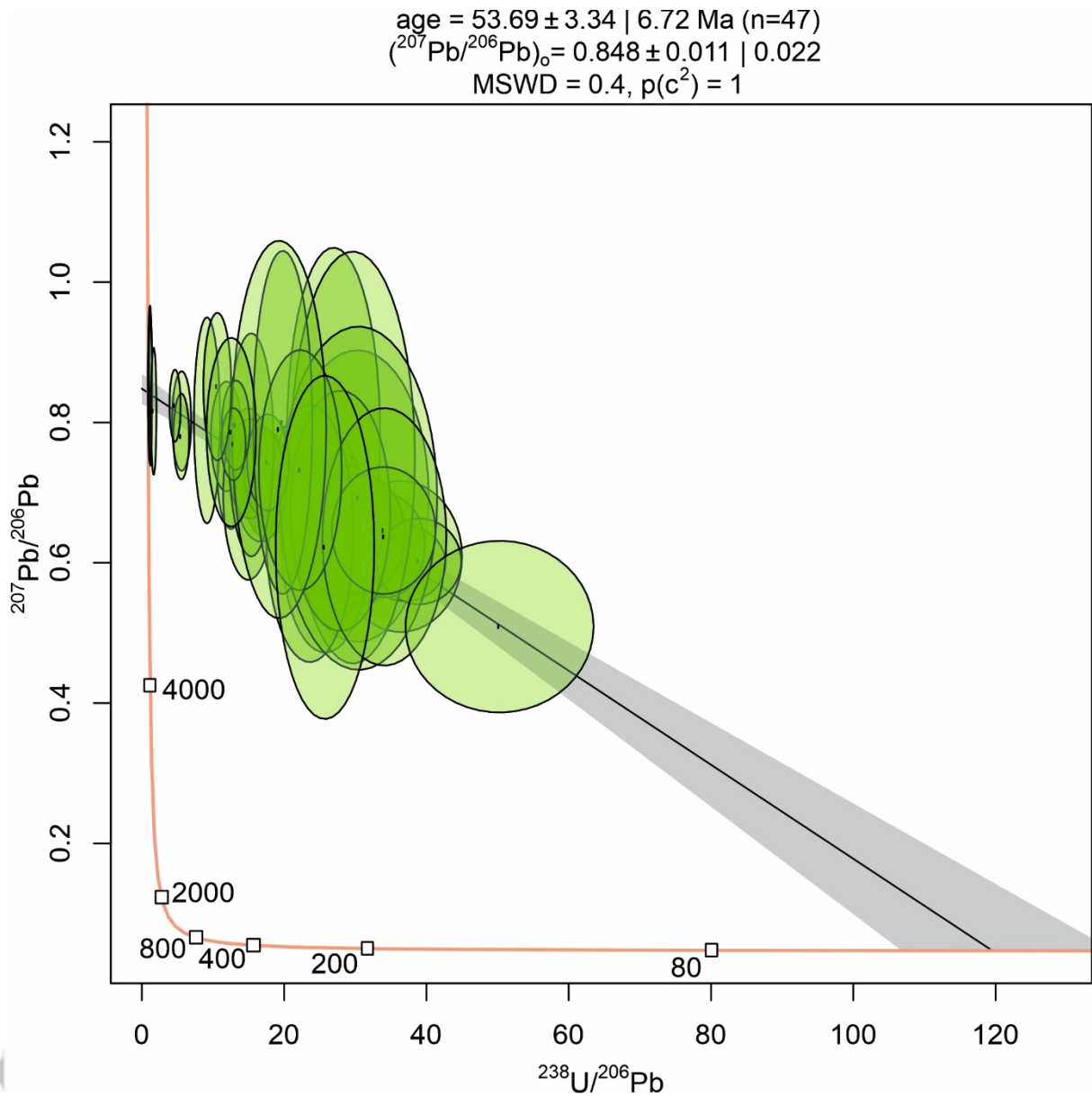
Fig. 4. Tera-Wasserburg diagram of the lacustrine carbonate sample CJC07.
