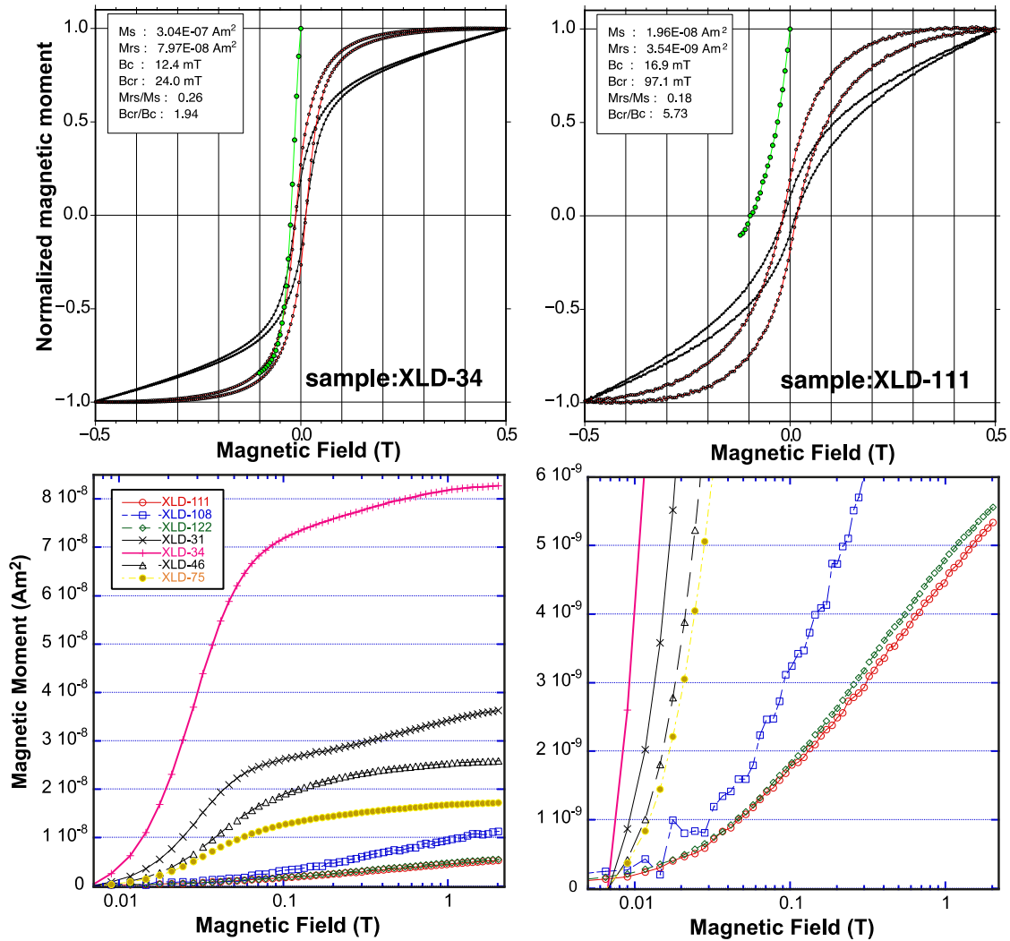
Fig. 6. High-field magnetic properties. Top) examples of hysteresis plots (black lines) for two samples of the Ledu section with magnetite (left) and hematite (right) as the dominant magnetic carrier, both showing a wasp-waisted loop. Red lines show the paramagnetic correction and green lines show the remanent curve. Bottom) IRM acquisition for seven samples of the Ledu section. The plot on the right is a zoom to highlight the low amount of magnetization acquired below 0.1 T in samples at the base of the Ledu section (XLD-108, XLD-111, XLD-122).
