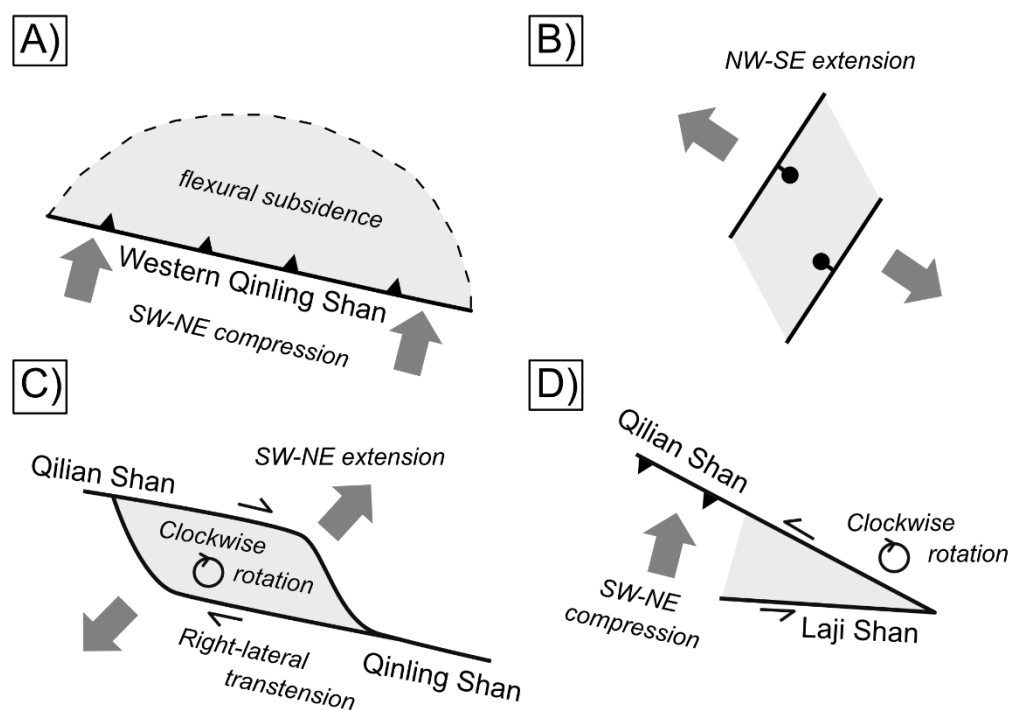
Fig. 11. Tectonic models for the origin of the Xining Basin: A) Foreland basin of the Western Qinling Shan (Fang et al., 2003; 2016; He et al., 2021; Liu et al., 2013). B) Extensional basin due to normal faulting (Fan et al., 2019). C) Right-lateral transtensional basin due to SW-NE extension (Wang et al., 2013; 2016). D) Left-lateral transtensional basin due to differential rotation of crustal blocks (Zhang et al., 2016).
