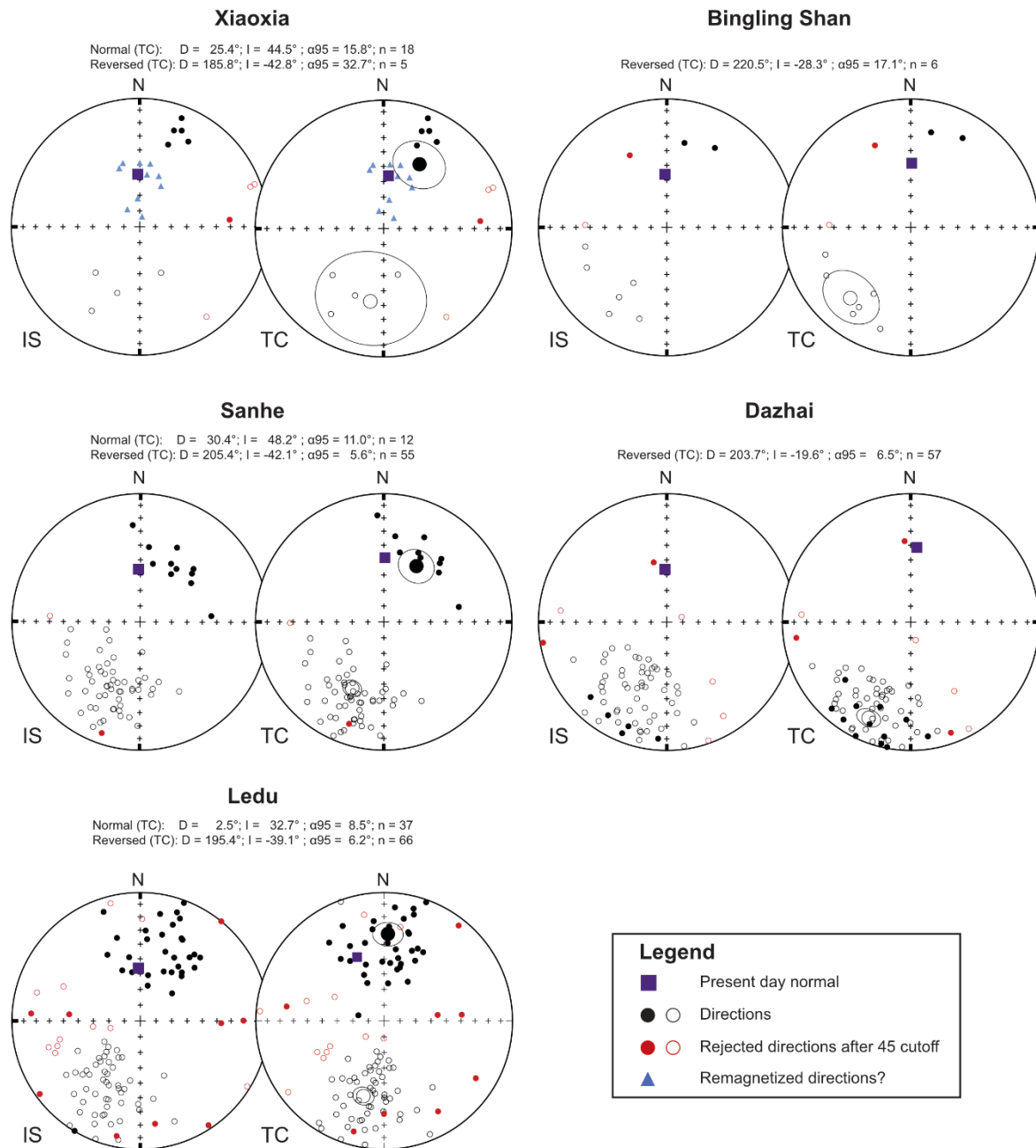
Fig. 7. Equal-area stereographic projections of calculated ChRM directions of the studied sections both in situ (IS) and tilt corrected (TC).
