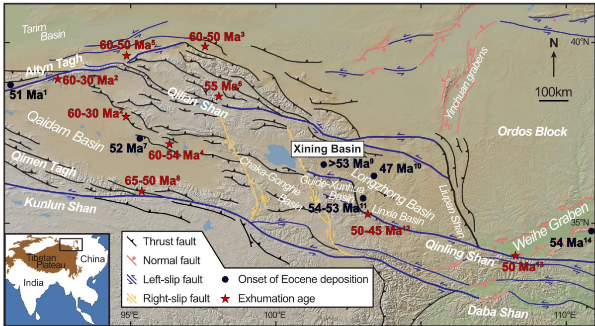
Fig. 10. Map of the northeastern Tibetan Plateau showing tectonic events during the early Eocene: 1) Li et al. (2018); 2) Jolivet et al. (2001); 3) He et al. (2017); 4) He et al. (2018); 5) He et al. (2020); 6) Li et al. (2020); 7) Ji et al. (2017); 8) Staisch et al. (2020); 9) He et al. (2021) and this study; 10) Wang et al. (2016); 11) Feng et al. (2021); 12) Clark et al. (2010); 13) Liu et al. (2013); 14) Chen et al. (2021). Modern-day topographic base map is from the GeoMapApp software (Ryan et al., 2009) available at http://www.geomapapp.org/ . The faults are redrawn from Zuza et al. (2016) and references therein.
