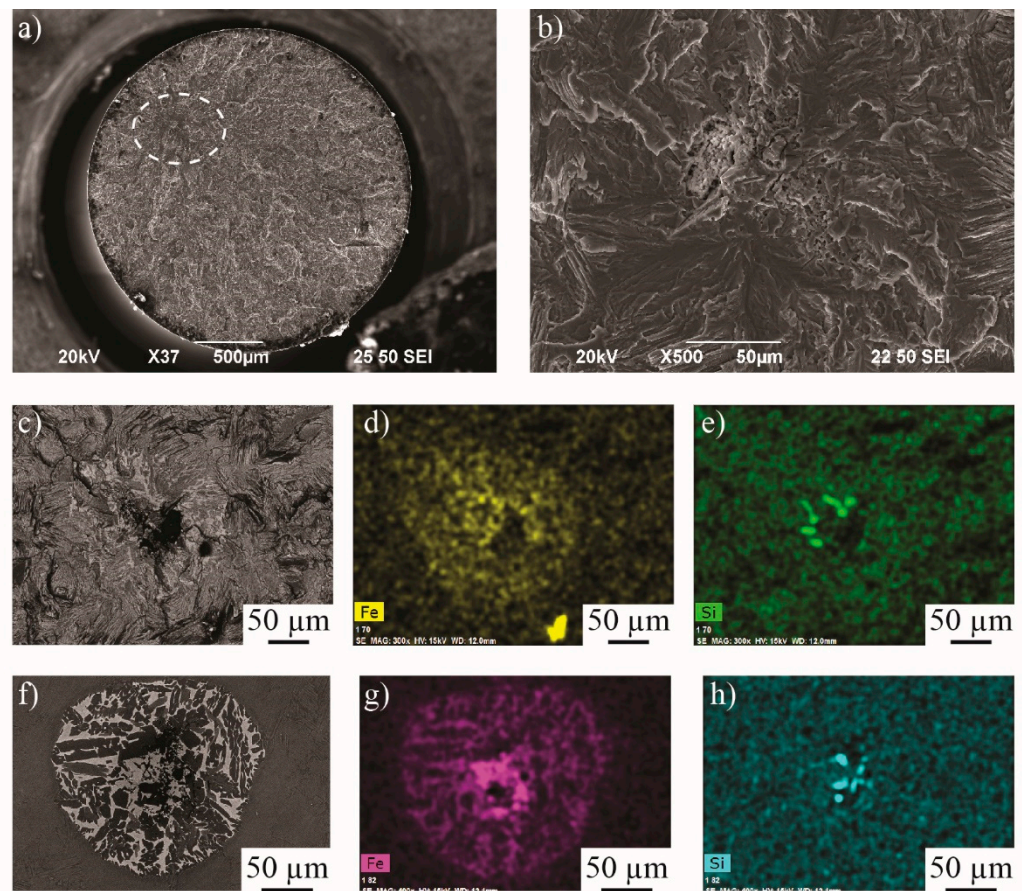
Figure 6. SEM analysis of a TNM + tensile sample densified at 1325 °C after rupture at room temperature (a–e) and comparison to a sample free of deformation (f–h). (a) Overview of the sample section with the crack initiation site circled; (b) enlargement of the site; (c) back-scattered electron image of the very centre of the initiation site; (d) corresponding EDX mapping of Fe; (e) corresponding EDX mapping of Si; (f) contaminated particle in a non-deformed sample taken from an as-SPSed billet of the TNM + alloy consolidated at 1325 °C; (g) corresponding EDX mapping of Fe; and (h) corresponding EDX mapping of Si.
