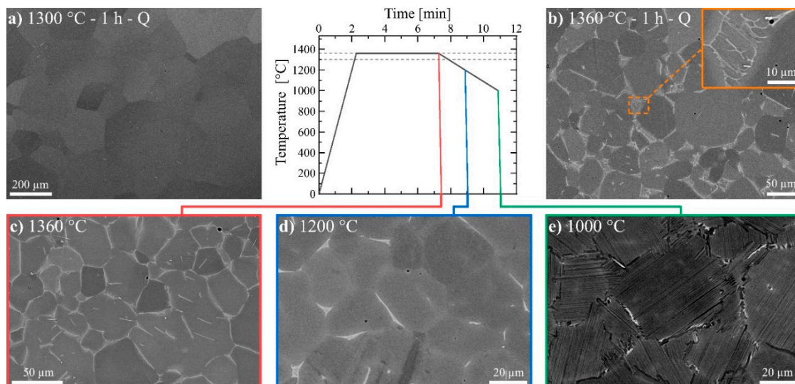
Figure 4. Microstructures of the TNM + alloy after various heat treatments: (a,b) correspond to 1 h heat treatments followed by quenching; (c–e) quenching from specific temperatures during the reproduced SPS cycle. The temperatures given in (c) through (e) mark the respective temperatures before the quenching to room temperature, e.g., see the time-temperature curve in the centre.
