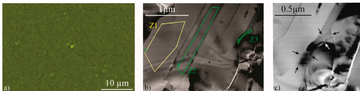
Figure 2. Study by SEM and TEM of the repartition of the Si atoms in the microstructure of the TNM + alloy densified at 1325 °C and within a silicide. (a) Si map by SEM of a large area; (b) delimitation of the three zones which were analysed (Table 4) and (c) TEM image of a \xi silicide precipitate.
