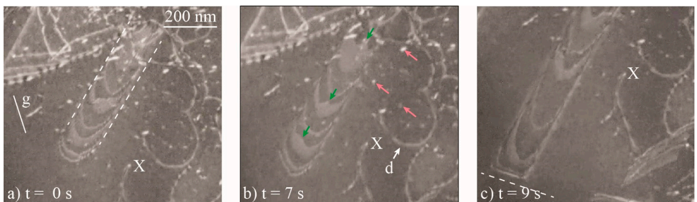
Figure 8. Progression of a mechanical twin in the \gamma phase of the TNM + alloy as observed by in situ tensile experiment in a TEM at room temperature. (a) Initial situation ( t = 0 s); (b) progression of the twin; and (c) blocking of the twin against another out-of-contrast twin whose direction is indicated by the white dotted line.
