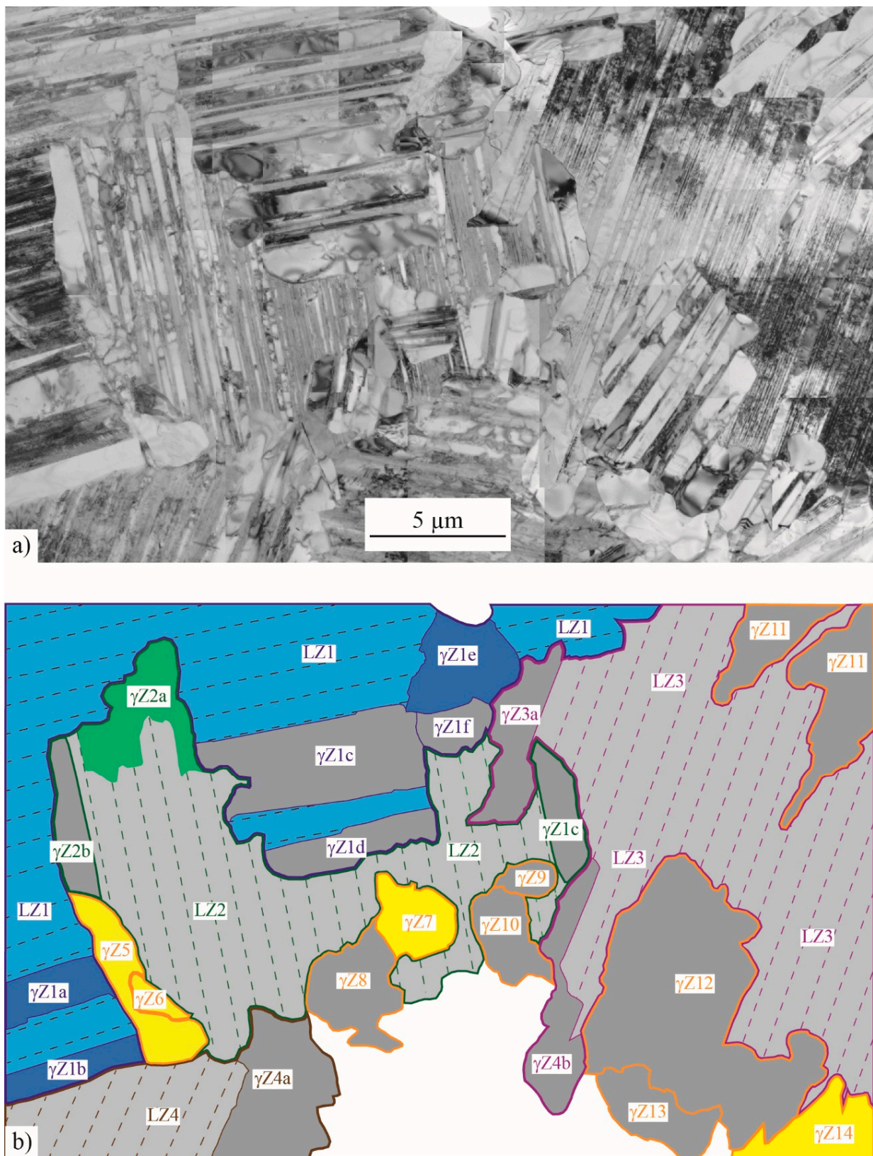
Figure 9. Post-mortem analysis of a 595 \mu\text{m}^2 area of a TNM + specimen by TEM. (a) Bright field image of the area; and (b) schematic drawing of the same area on which is indicated the type of microstructural feature (LZ for lamellar zones, \gamma\text{Z} for \gamma grains). See text for the explanation of the colour code. The white area has not been analysed.
