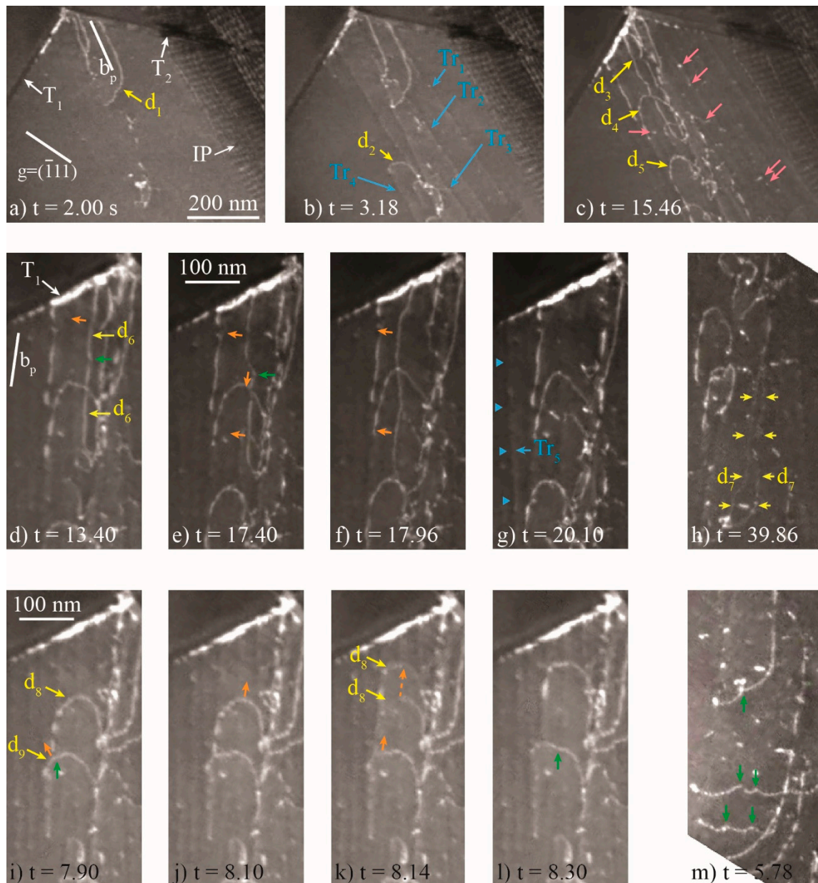
Figure 7. Movements of ordinary dislocations and formation of slip traces in the \gamma phase of the TNM + alloy as observed by in situ tensile tests at room temperature in a TEM. (a–c) global movements of several ordinary dislocations and formation of several traces; (d–i) glide of a screw dislocation d_6 ; (h) illustration of the rapidity of the movement through the observation of the initial and final positions of a jump on the same frame; (i–l) glide of two non-screw dislocations d_8 and d_9 ; and (m) pinning points on non-screw segments. g is the direction of the diffraction vector used for the images. b_p is the projection of the Burgers vector ( b = a/2[\bar{1}10] ) in the observation plane. See text for details about other indications reported in this figure and about the description of the movements. The times which are reported are those of the video.
