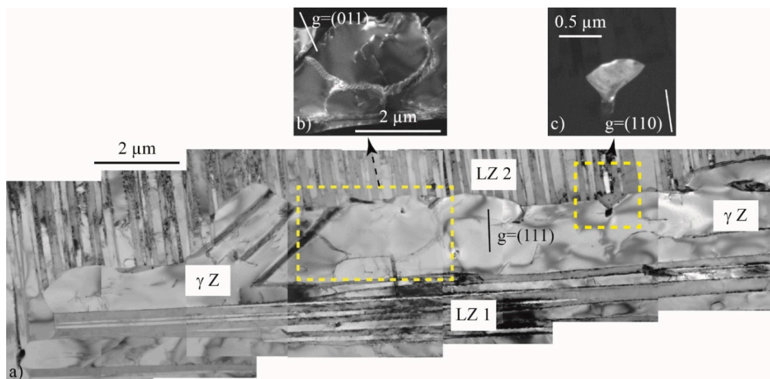
Figure 3. TEM study in TNM + of a \gamma zone ( \gamma Z ) situated between two lamellar zones labelled LZ1 and LZ2. (a) General view in bright field mode; (b) ordered domain in dark field mode; and (c) \beta_o precipitates in dark field mode.
