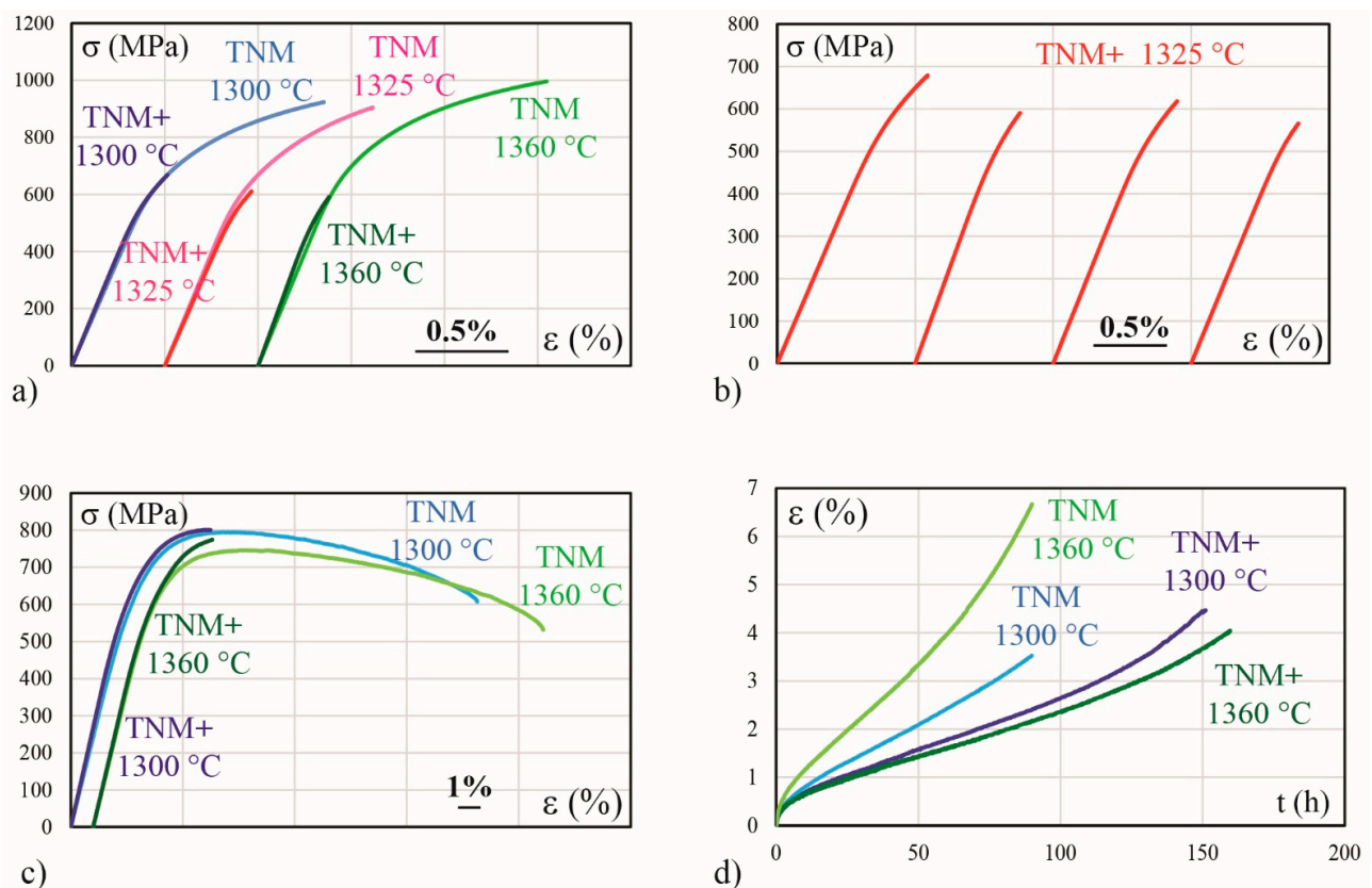
Figure 5. Mechanical properties of the TNM + and TNM alloys. (a) Comparison of the tensile tests at room temperature performed on the two alloys for three different dwell temperatures; (b) results of four tensile tests performed at room temperature on TNM + samples sintered at 1325 °C; (c) comparison of the tensile curves recorded at 800 °C for the TNM + and TNM alloys which were densified at different dwell temperatures; and (d) creep curves at 800 °C under 200 MPa. All temperatures indicated in the diagrams are the dwell temperatures used for the densification of the corresponding material. The tensile curves are shifted by 0.5% or 1% so that they differ from each other.
