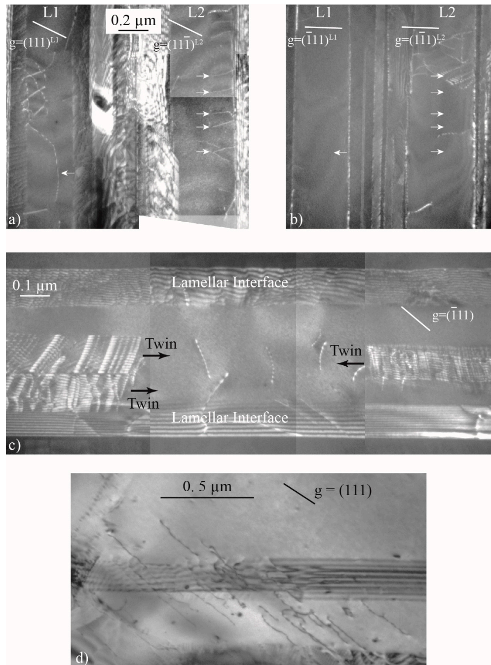
Figure 10. Several examples of deformed zones in thin foils extracted from TNM + specimens, which were deformed at room temperature. (a,b) Lamellae oriented in soft mode containing some ordinary dislocations which have glided in a plane parallel to the interface plane; (c) twins in a lamella oriented in soft mode; and (d) ordinary dislocations and a deformation twin in a \gamma zone of a border.
