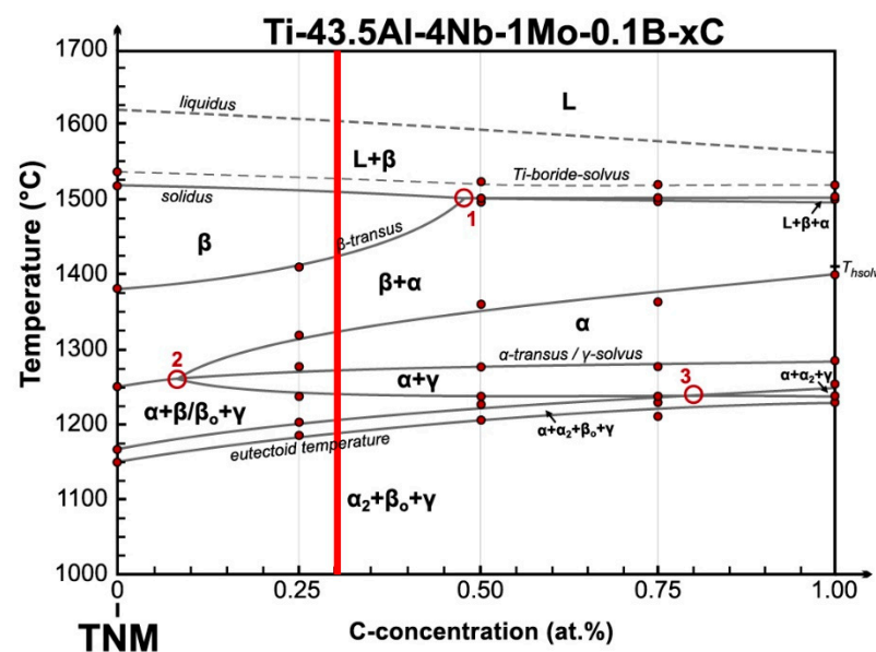
Figure 11. Quasi-binary phase diagram of the Ti-43.5Al-4Nb-1Mo-0.1B-xC (at.%) system as determined by Schwaighofer et al. [24]. The red line indicates the C content of the studied TNM + alloy. Adapted with permission from Ref. [24].
