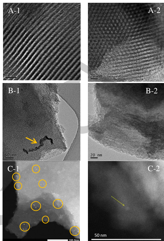
Figure 1. HRTEM micrographs of SBA-PrSH y ·Pd x materials (A-1: y=6 and A-2: y=65) and SBA-PrSH 10 ·Pd y materials (B-1: y=6 and B-2: y=65). HAADF-STEM micrographs of SBA-PrSH y ·Pd x materials (C-1: y=6 and C-2: y=65). Palladium nanoparticles aggregate is indicated by a yellow arrow (B-1) and isolated palladium nanoparticles are highlighted by yellow circles (C-1)
