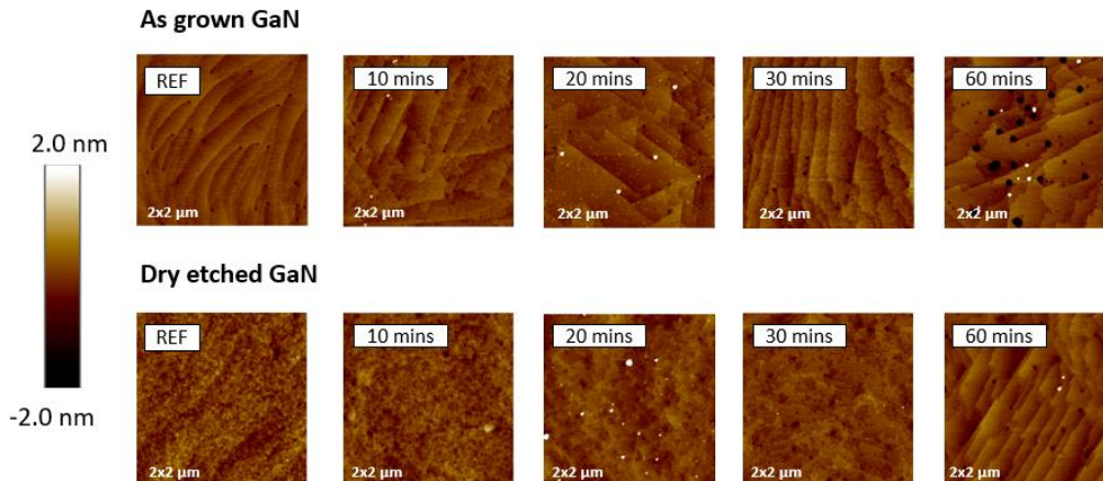
Figure 6. AFM images before and after hot H 3 PO 4 treatment at different durations
