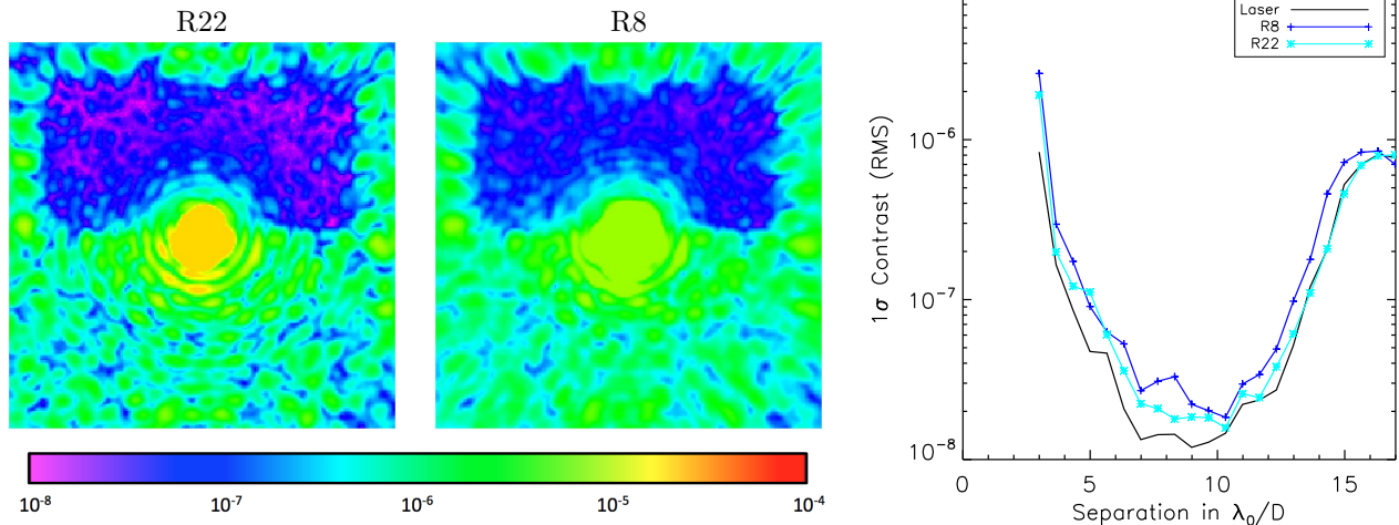
Figure 10. Left: the two images obtained in wide bandpass filters (Table 1) with the DZPM. We control the DM using the command obtained with DZPM+SCC in monochromatic light. Right: Associated 1\sigma contrast curves compared to the performance obtained in monochromatic light (black solid line).
