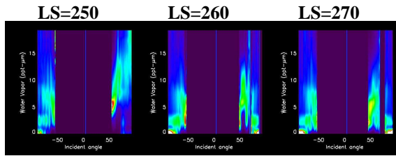
Figure 1: Water Vapor distribution over the incidence angle for the three LS= 250°,260° and 270°. Negative values indicate morning values. It is visible a constant increase of the water vapor in all the three images moving from -90° to +90° (more evident in LS=250° and less evident for LS=270°). This shows a non correlation between the water vapor variability and the incidence angle, which implies that scattering is not the main cause of the water vapor variability.
