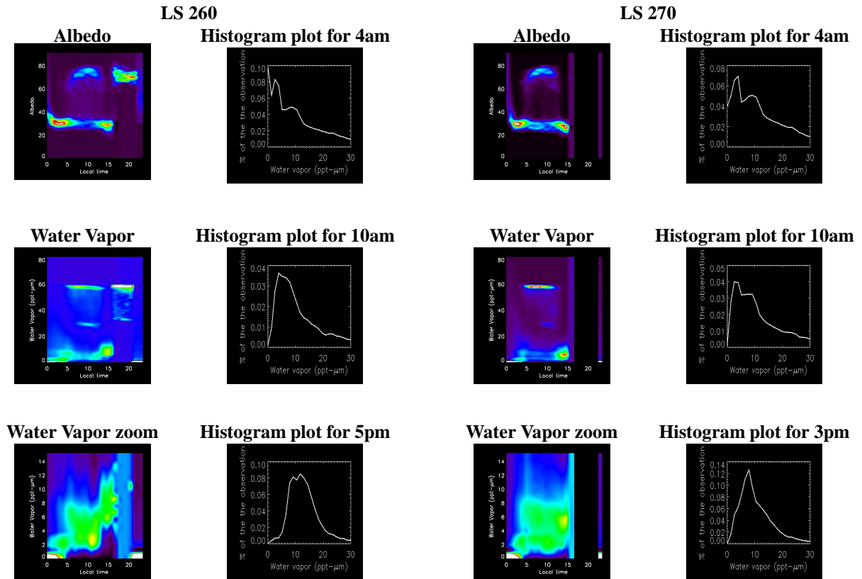
Figure 3: As for LS=250°, but data represent LS=260°. Histograms of the water vapor show selected local times (4am, 10am and 5pm). The albedo presents a constant value of 0.35; a small increase is detected in the morning (~38%). The higher values from 7am to 12pm is due to the presence of the CO 2 ice, observations over the ice cap. Water Vapor second group (30ppt- \mu m) shows an increase for values between 4pm and 8pm, this should be taken very carefully because could be due to a very small contamination of CO 2 .
