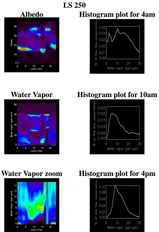
Figure 2: On the left: Water vapor and Albedo maps for the period LS=250°. Color table shows the ratio of how many observations per local time has a selected value; each of these values are divided by the total number of observations per each local time. On the right: Histograms of the water vapor distribution for selected local times (4am, 10am and 4pm). The albedo presents a constant value of 0.35, with a little decreasing slope with time (inside the error bar). Slightly higher values after 8pm ( \sim 0.4 ) suggest the possible presence of ice on the ground, which, otherwise, has not been spectrally detected. The higher values from 7am to 1pm is due to the presence of the CO 2 ice present in the ice cap. Water Vapor can be divided in three groups: values ranging between 0 and 15 ppt- \mu\text{m} , values around 30ppt- \mu\text{m} and values above 30ppt- \mu\text{m} . The first group (between 5am and 4pm) increases and it is noticeable like values under 2 ppt- \mu\text{m} in the morning and then 4 ppt- \mu\text{m} in the afternoon are not detected, which is the case for the early morning and the late afternoon. The second group seems to be correlated with the regions close to the CO 2 ice (but still free of ice), which may imply that ice cap is a main source of H 2 O. The third group is a detection of CO 2 ice, these values should not be interpreted as Water Vapor. This group is highly correlated with high albedo regions (from 50% to 80%, due to ice), which confirm the sensitivity of our method to the CO 2 ice.
